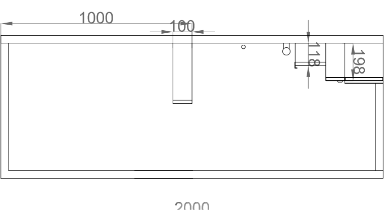
Proposed Side Elevation of Unit @ 1 : 20
