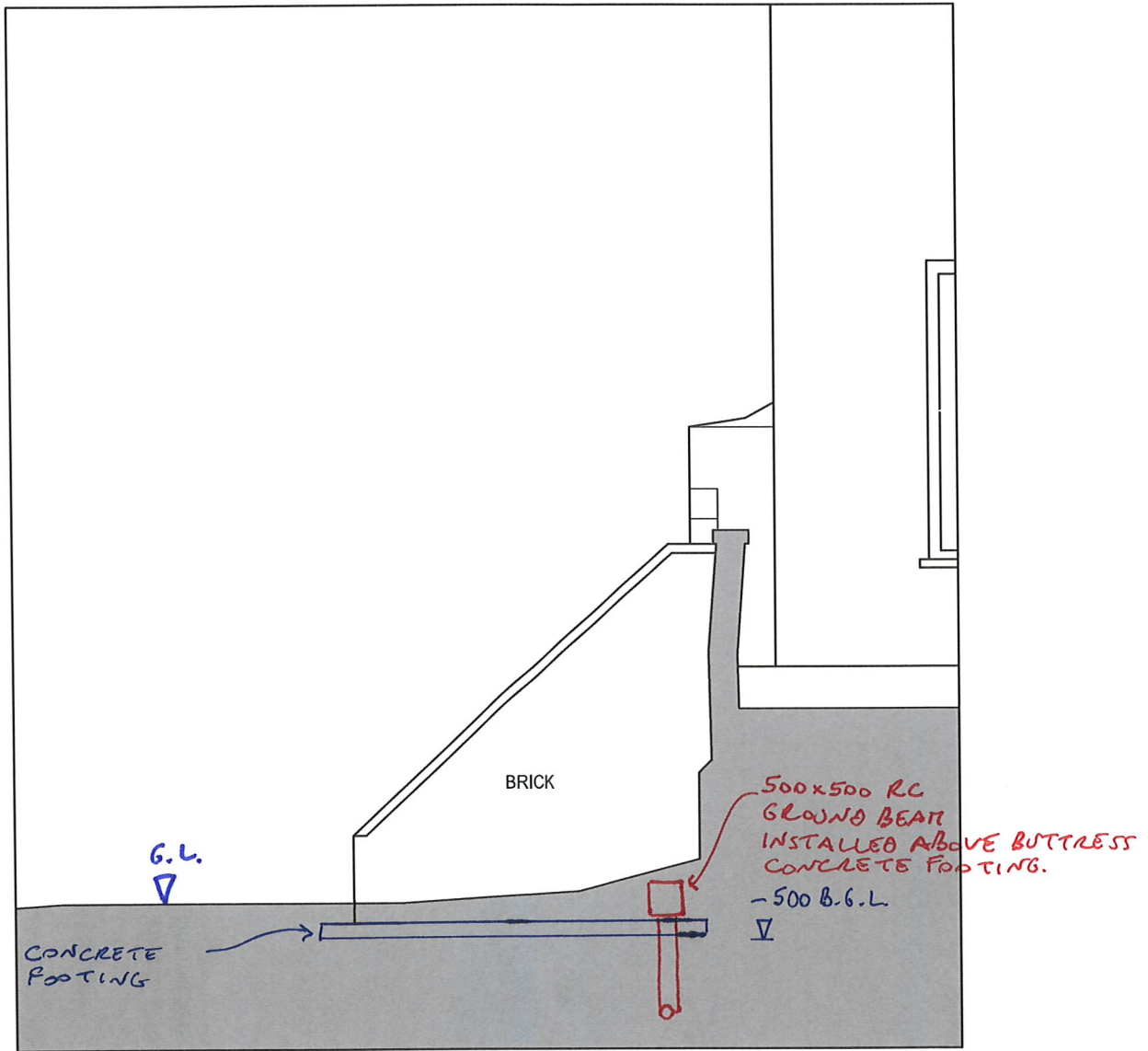
2 Section AA showing buttress 1:50 @ A1
