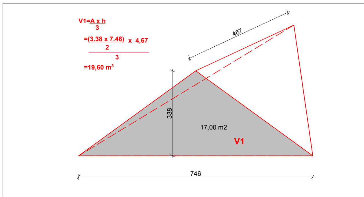
HIP TO GABLE VOLUME CALCULATION
