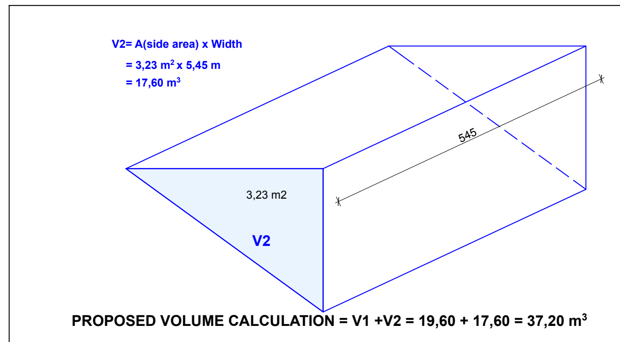
REAR DORMER VOLUME CALCULATION
