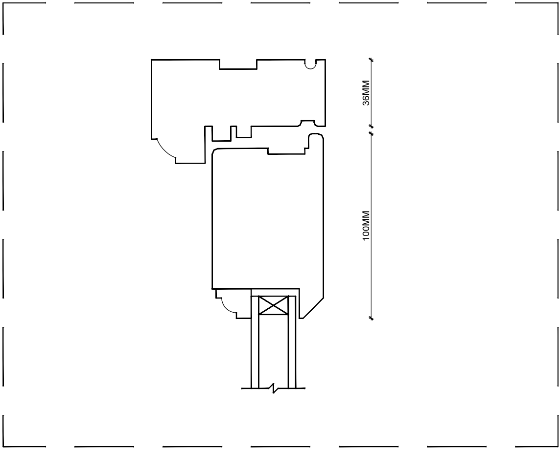
TOP FRAME DETAIL Scale 1:2 @ A2
