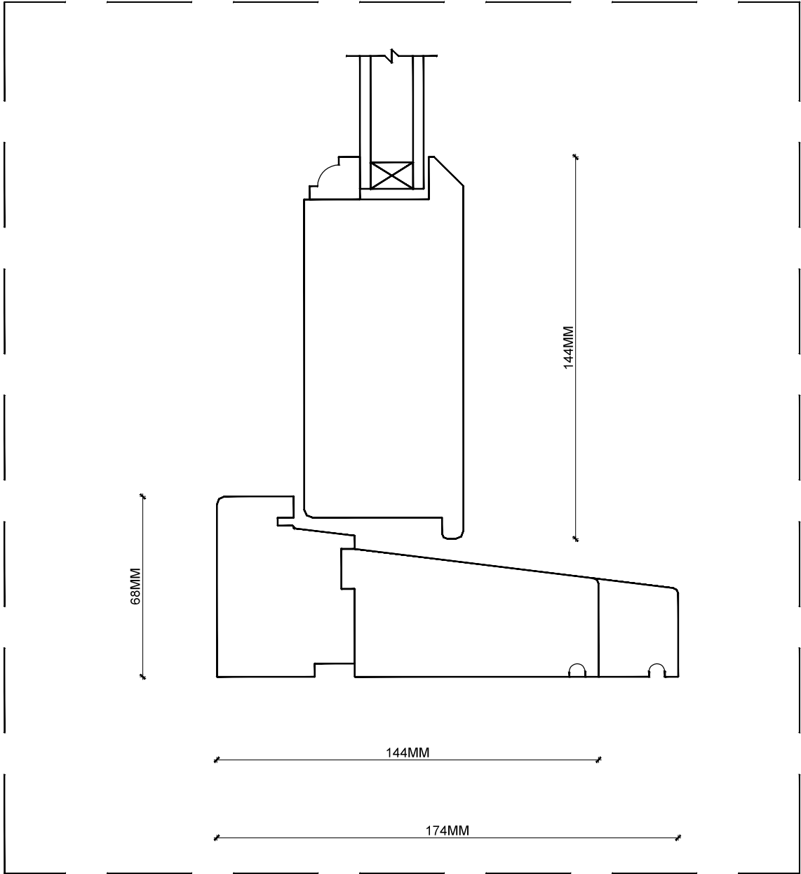
BOTOM FRAME DETAIL Scale 1:10 @ A2
