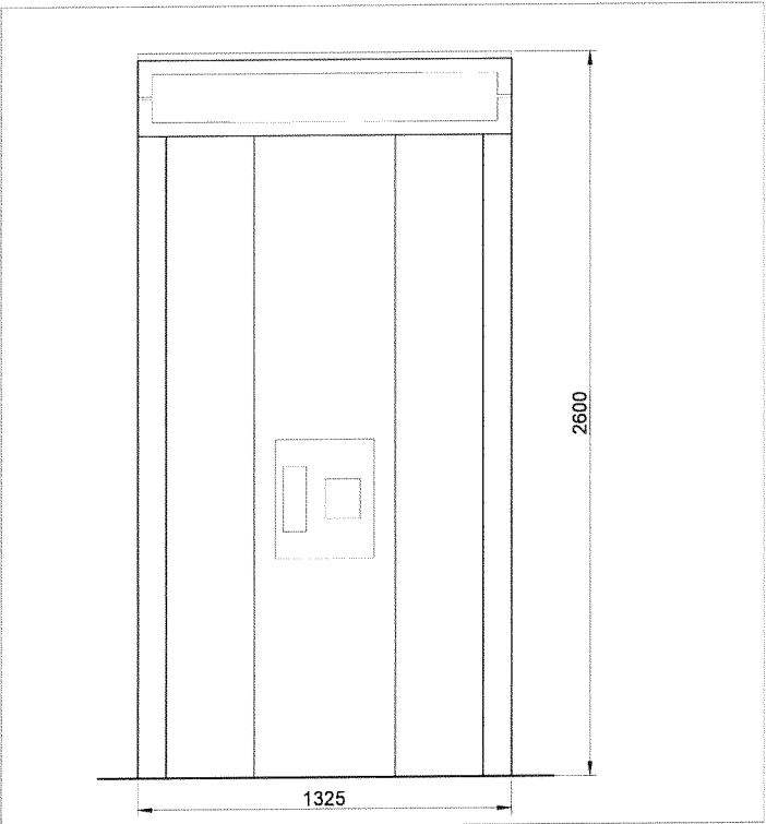
03 Front Elevation
