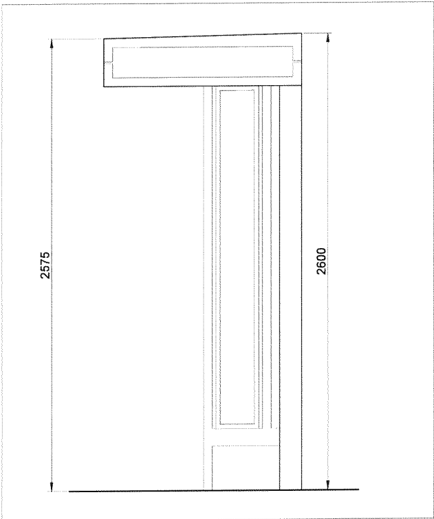
04 Side Elevation
