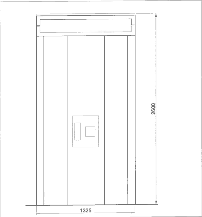
03 Front Elevation
