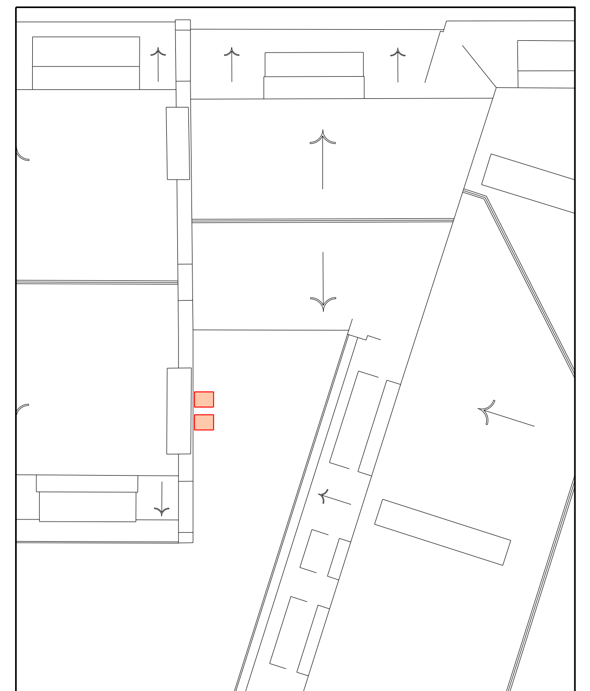
Roof Plan: Extract Ducts in Orange
