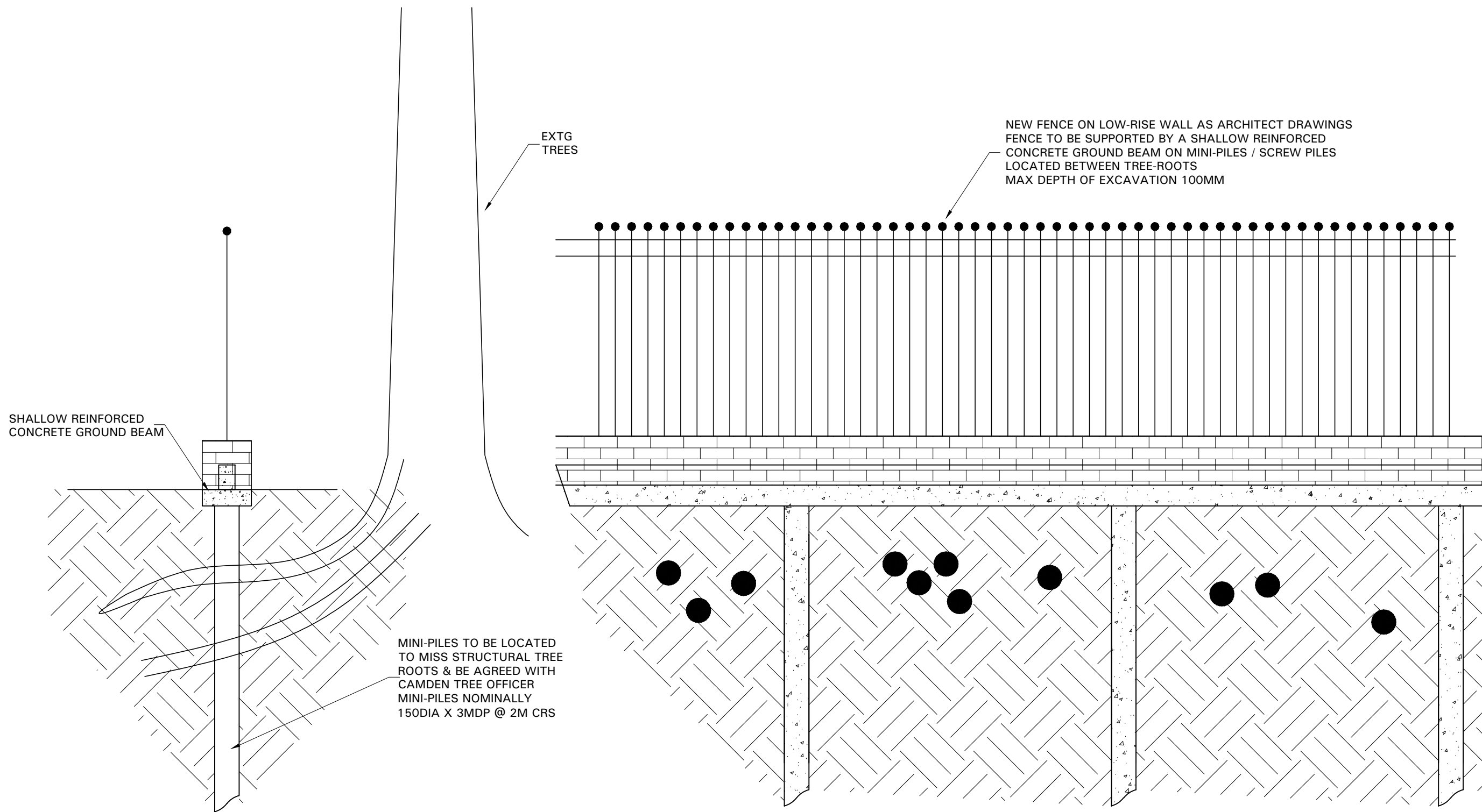
SECTIONAL ELEVATION
