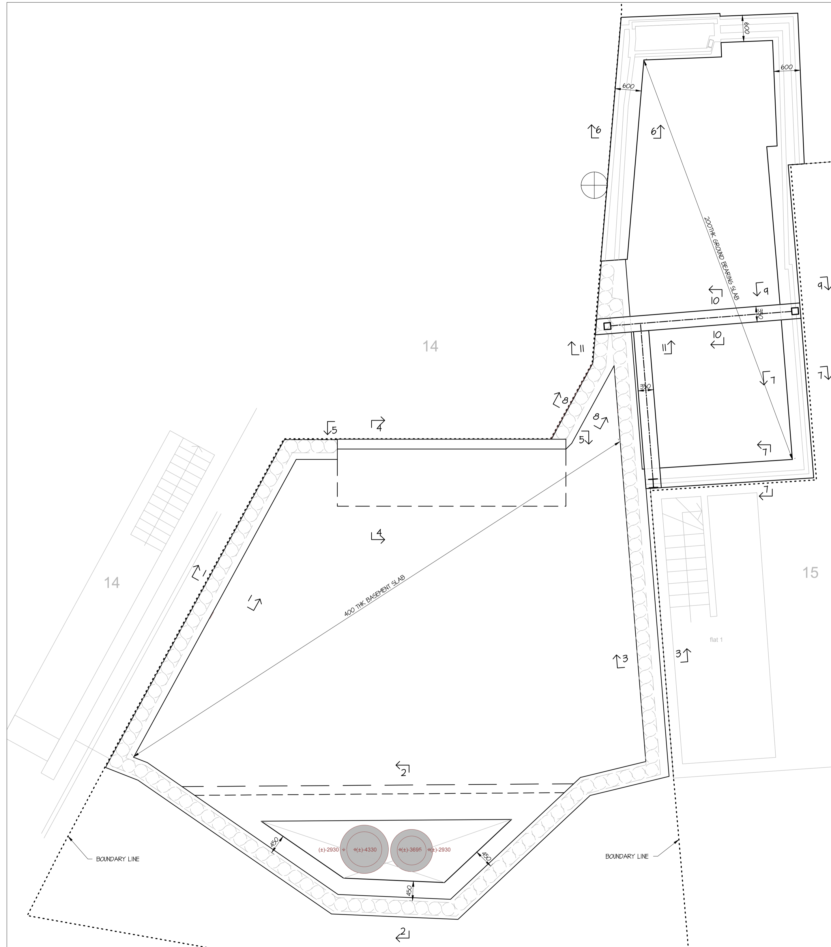
BASEMENT LAYOUT SCALE 1:50
