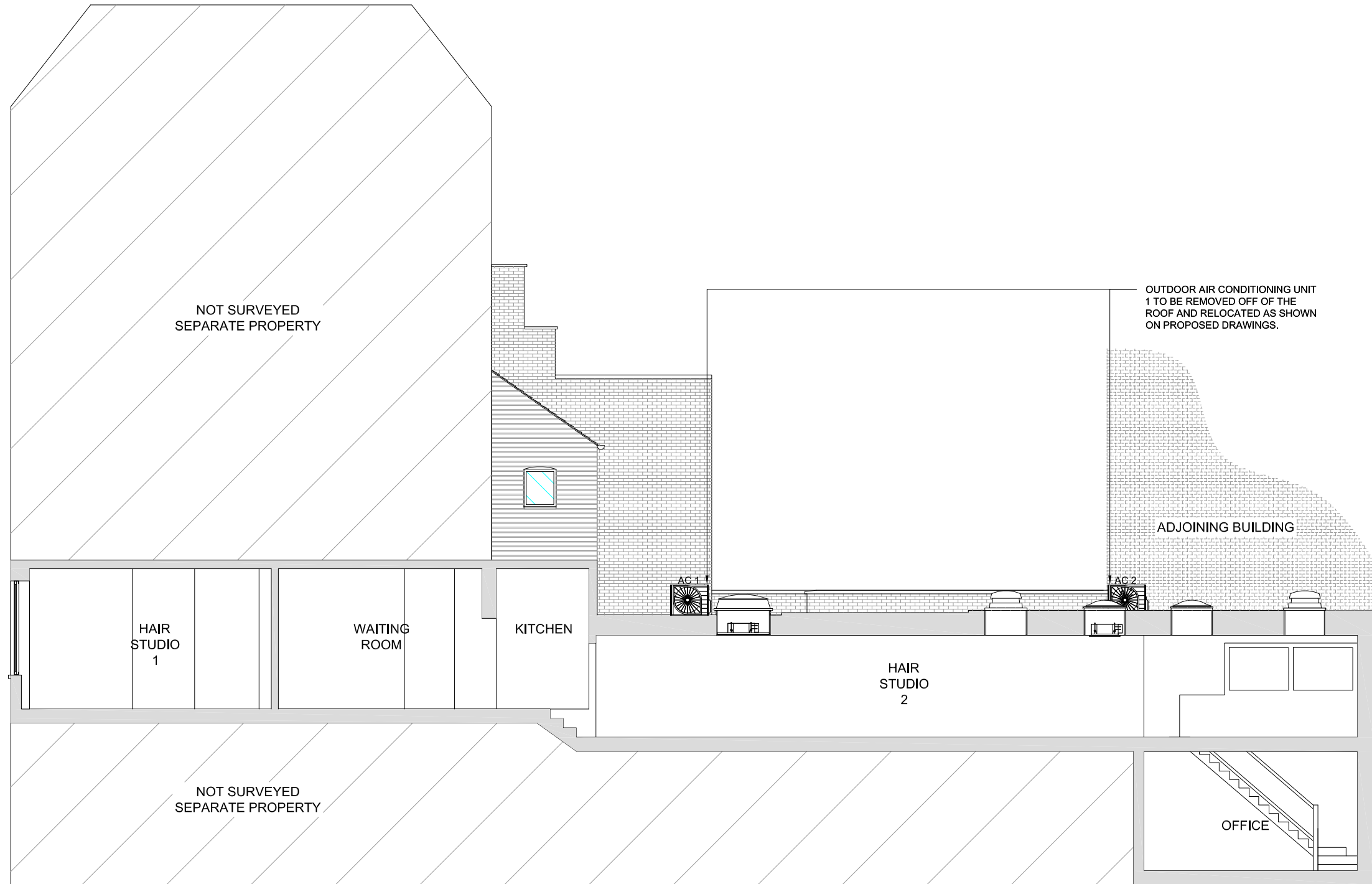
EXISTING SECTION
