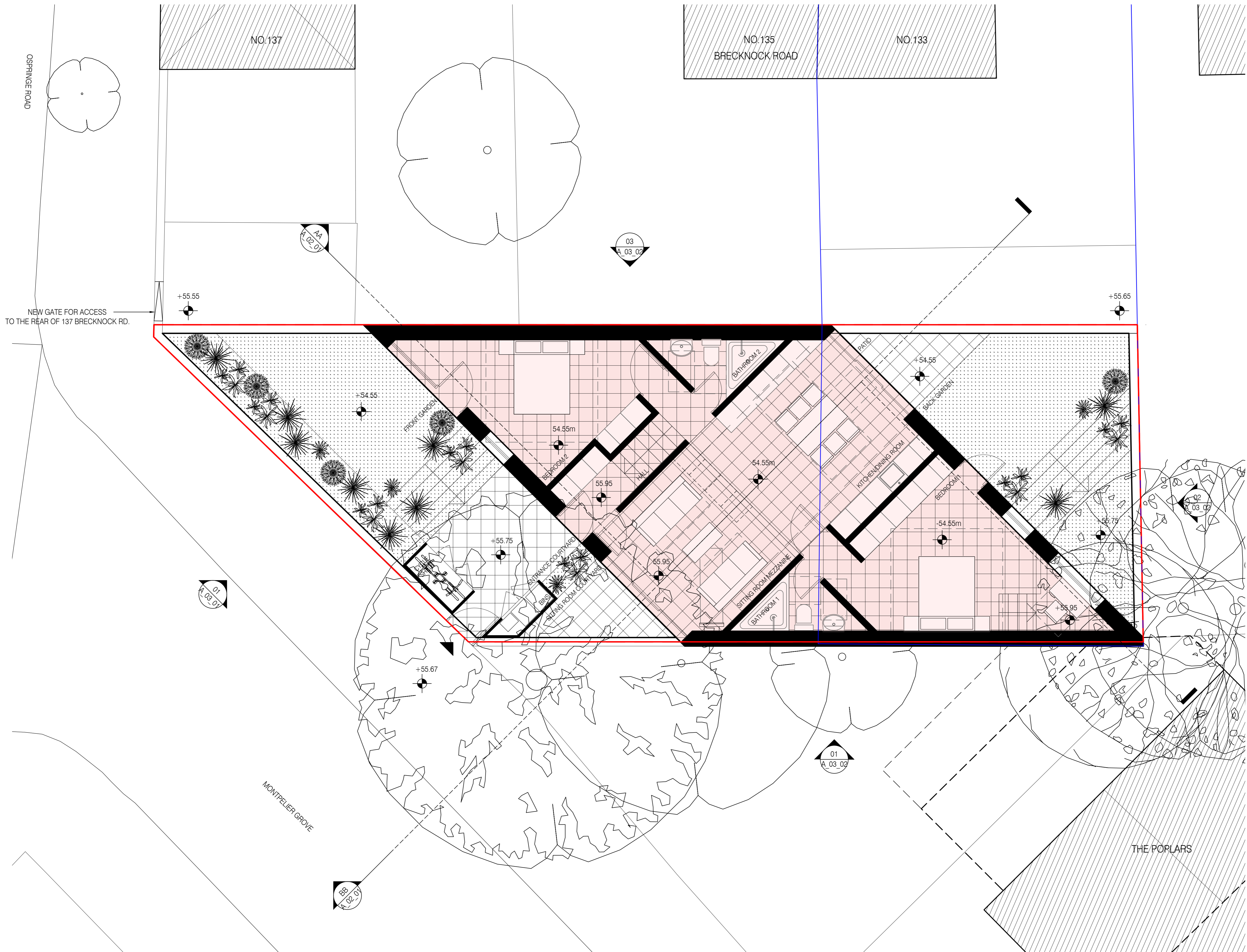
01 PROPOSED GROUND FLOOR PLAN SCALE: 1:50 @ A1 / 1:100 @ A3
