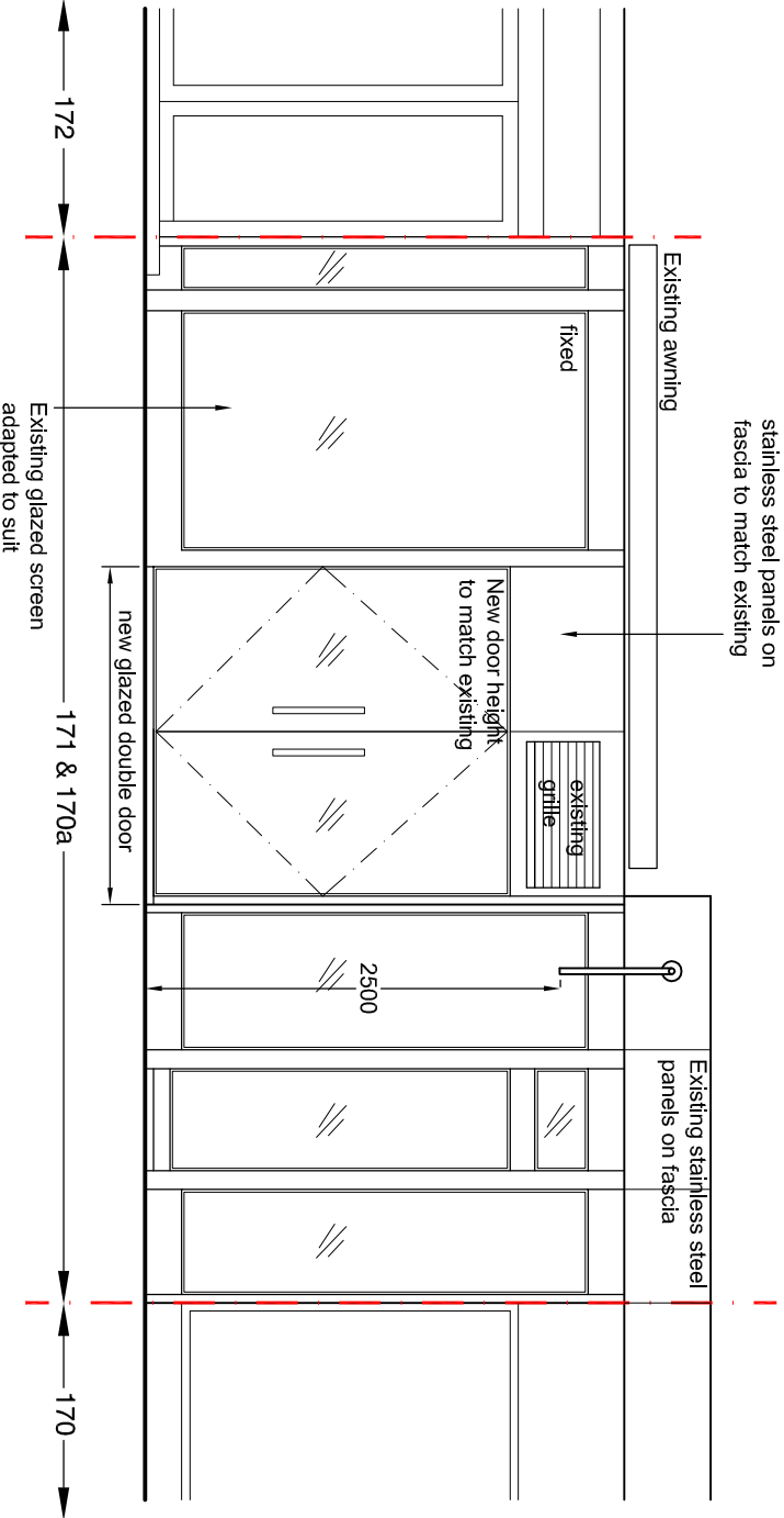
○ Proposed Shopfront Elevation Scale 1:50
