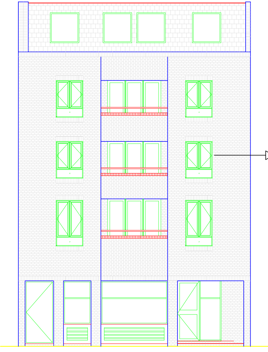
Proposed Front Elevation 1:100@A3
