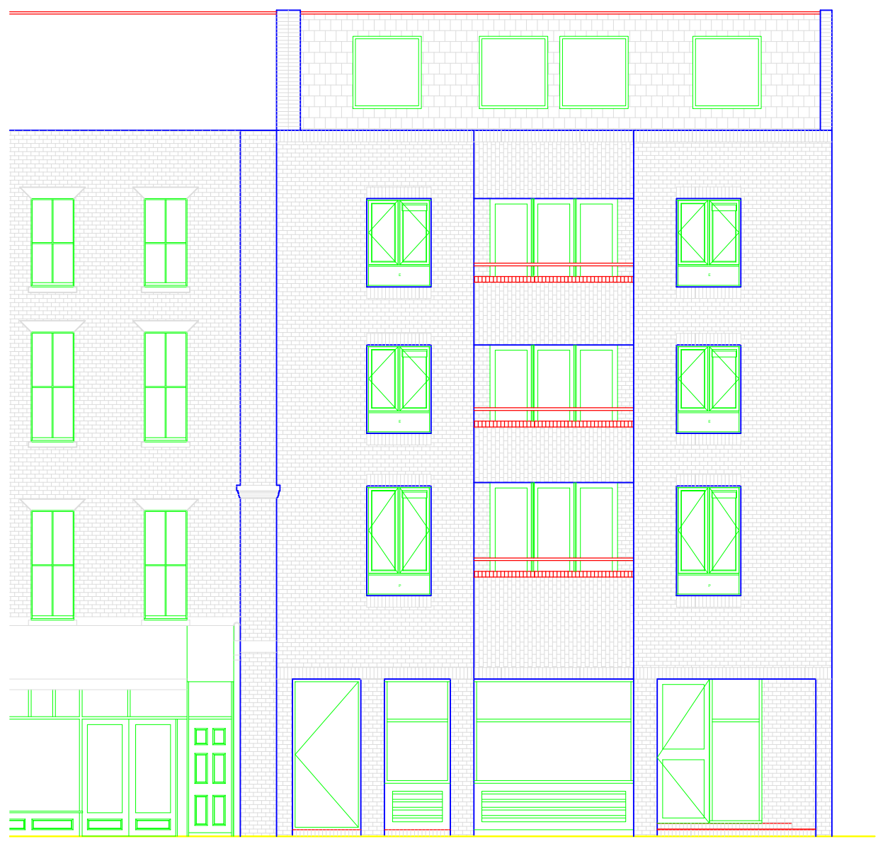
Existing Front Elevation 1:100@A3
