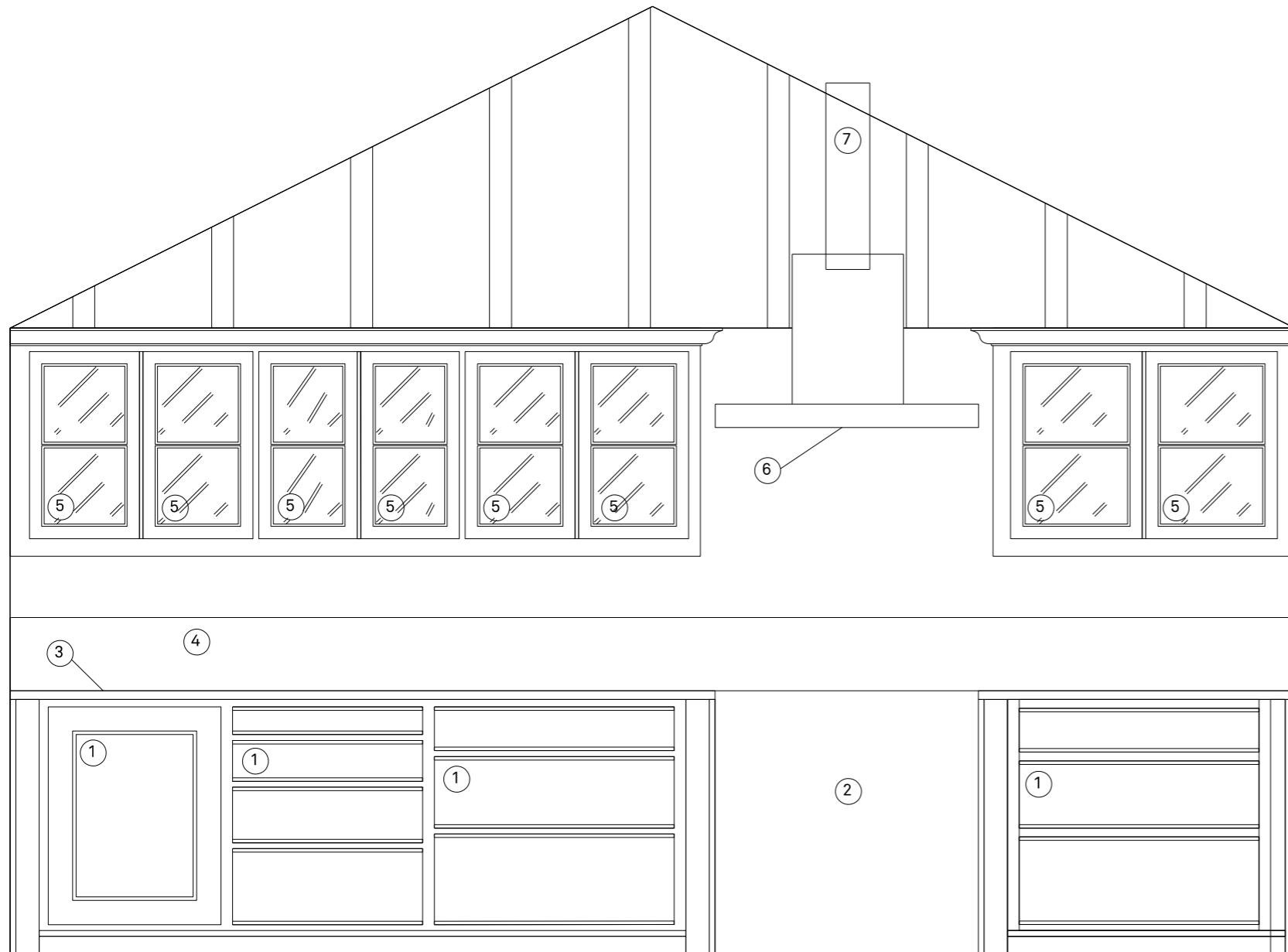
2 Kitchen Elevation 2 442
