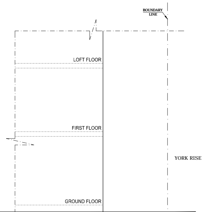
PRE-EXISTING SIDE ELEVATION SCALE: 1/100
