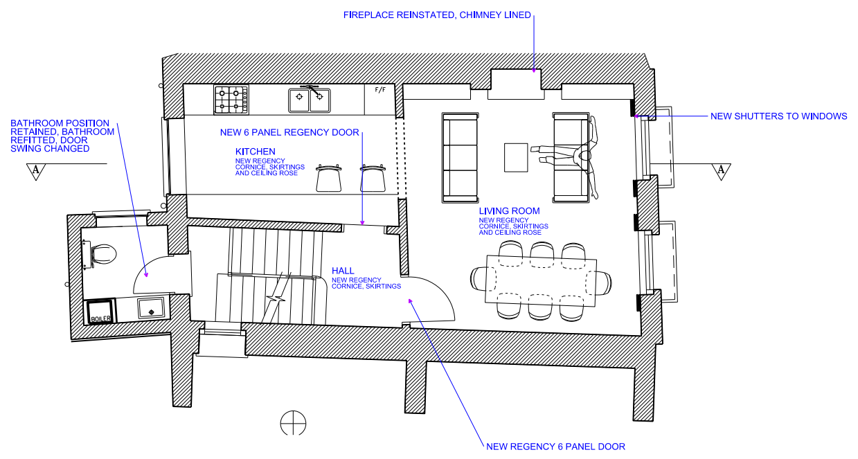
01 PROPOSED FIRST FLOOR PLAN
