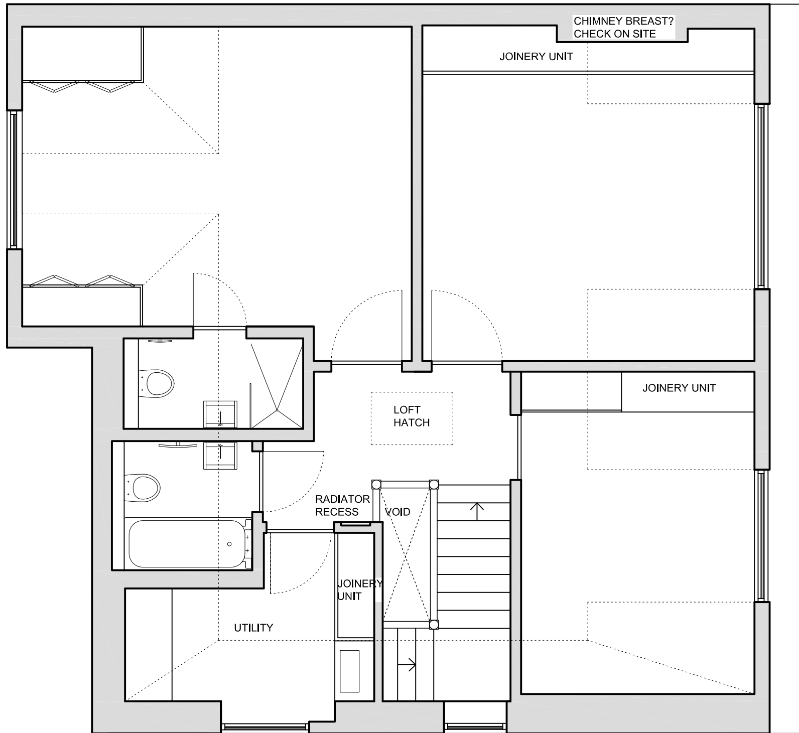
SECOND FLOOR
