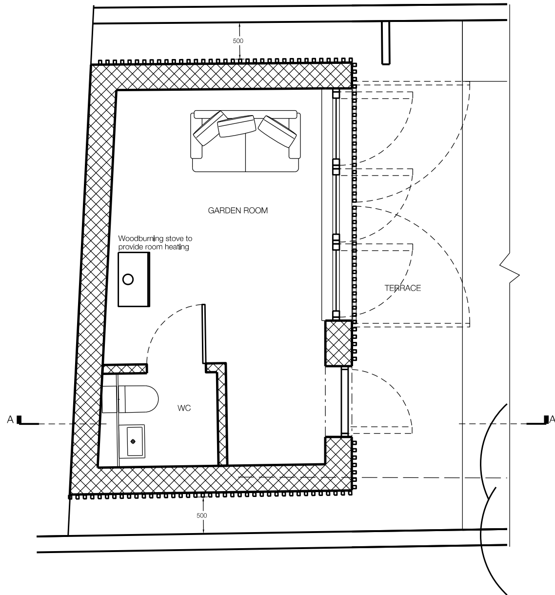
PROPOSED GARDEN ROOM FLOOR PLAN
