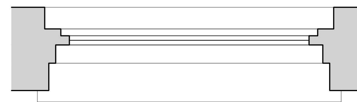
FF.05 Window type A Sash Window
