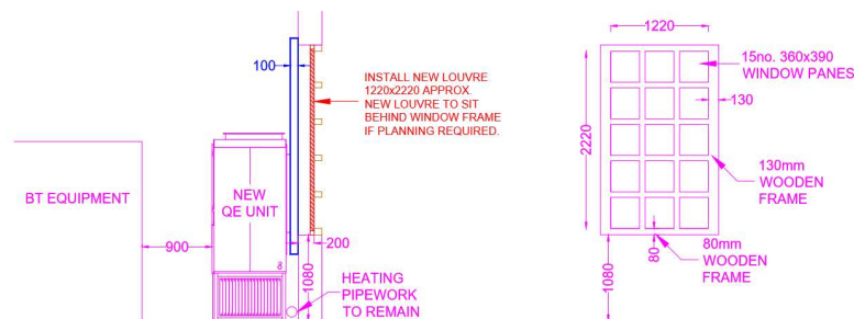
DETAIL 2: SIDE ELEVATION FOR UNIT POSITION & WINDOW LAYOUT
