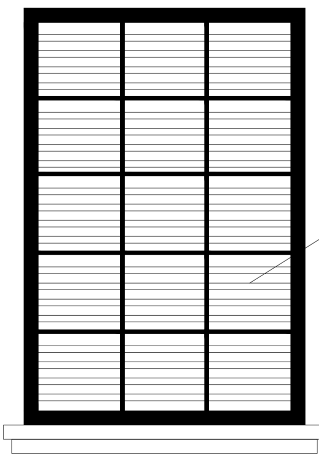
Louvre Detail 1:20
