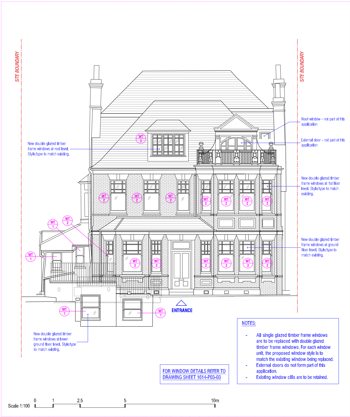
[01] PROPOSED NORTH ELEVATION
