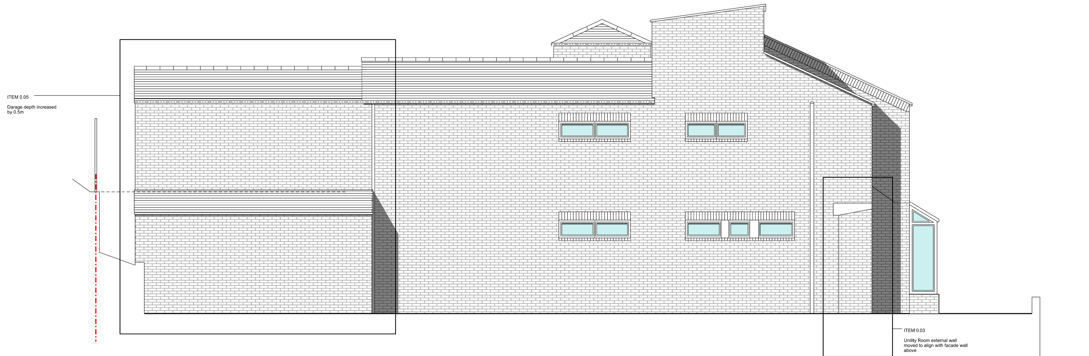
02 SIDE (EAST) ELEVATION AS PROPOSED KAM02_P_132 SCALE: 1:50 @ A1
