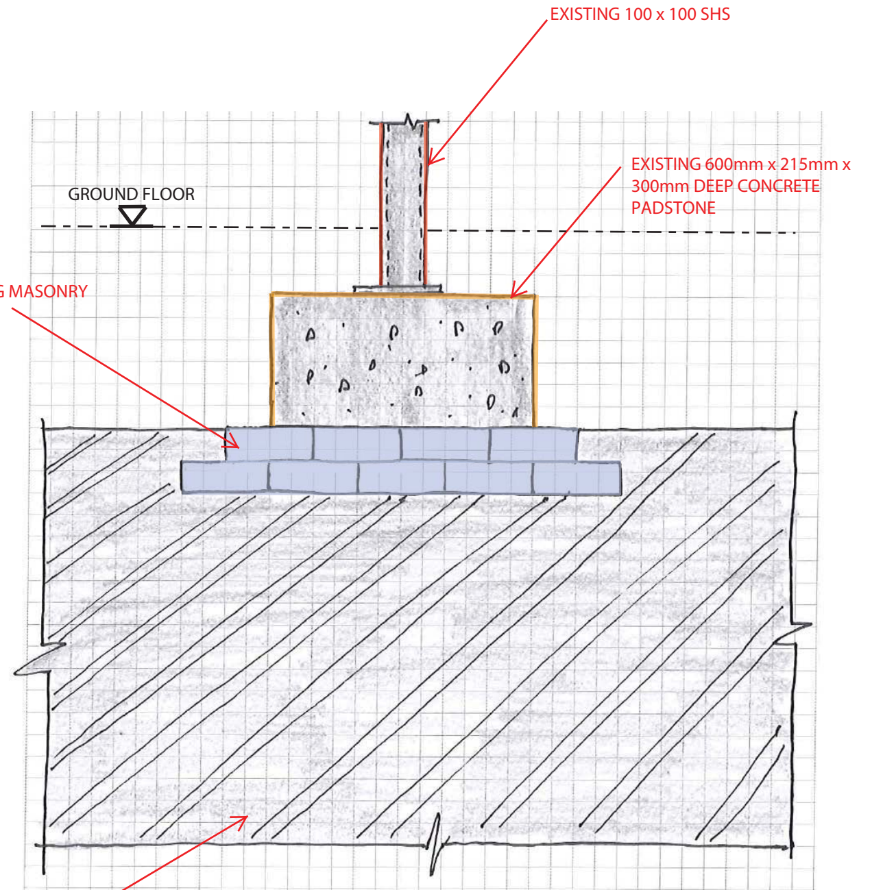
SECTION 1-1
