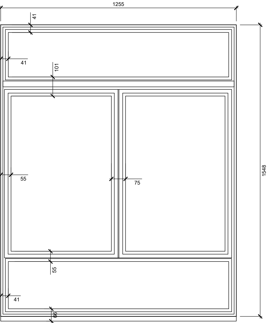
1 TYPICAL EXISTING WINDOW Scale: 1:10 @ A3
