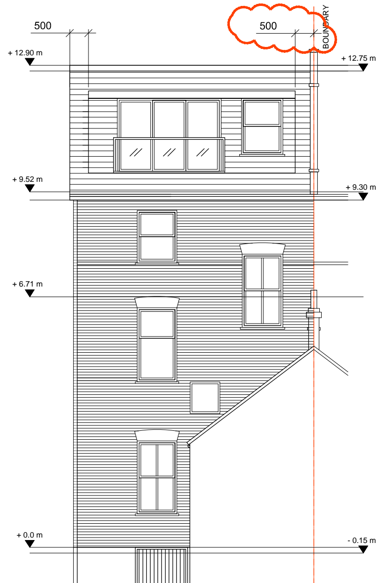
3 REAR ELEVATION - PROPOSED Scale: 1:100
