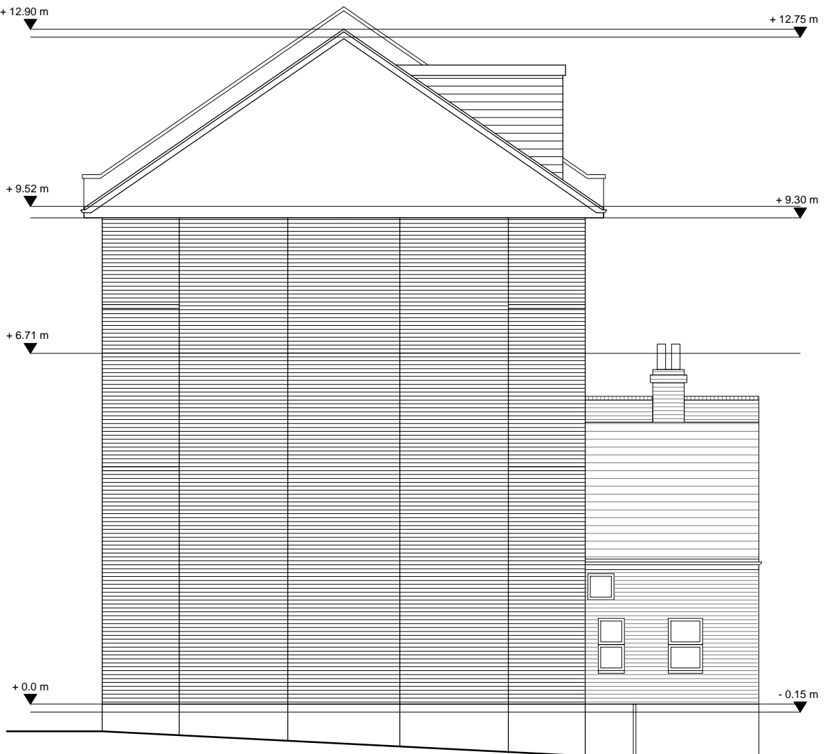
2 SIDE ELEVATION - PROPOSED Scale: 1:100
