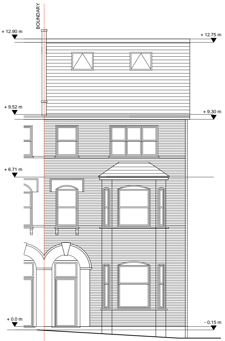
1 FRONT ELEVATION - PROPOSED Scale: 1:100
