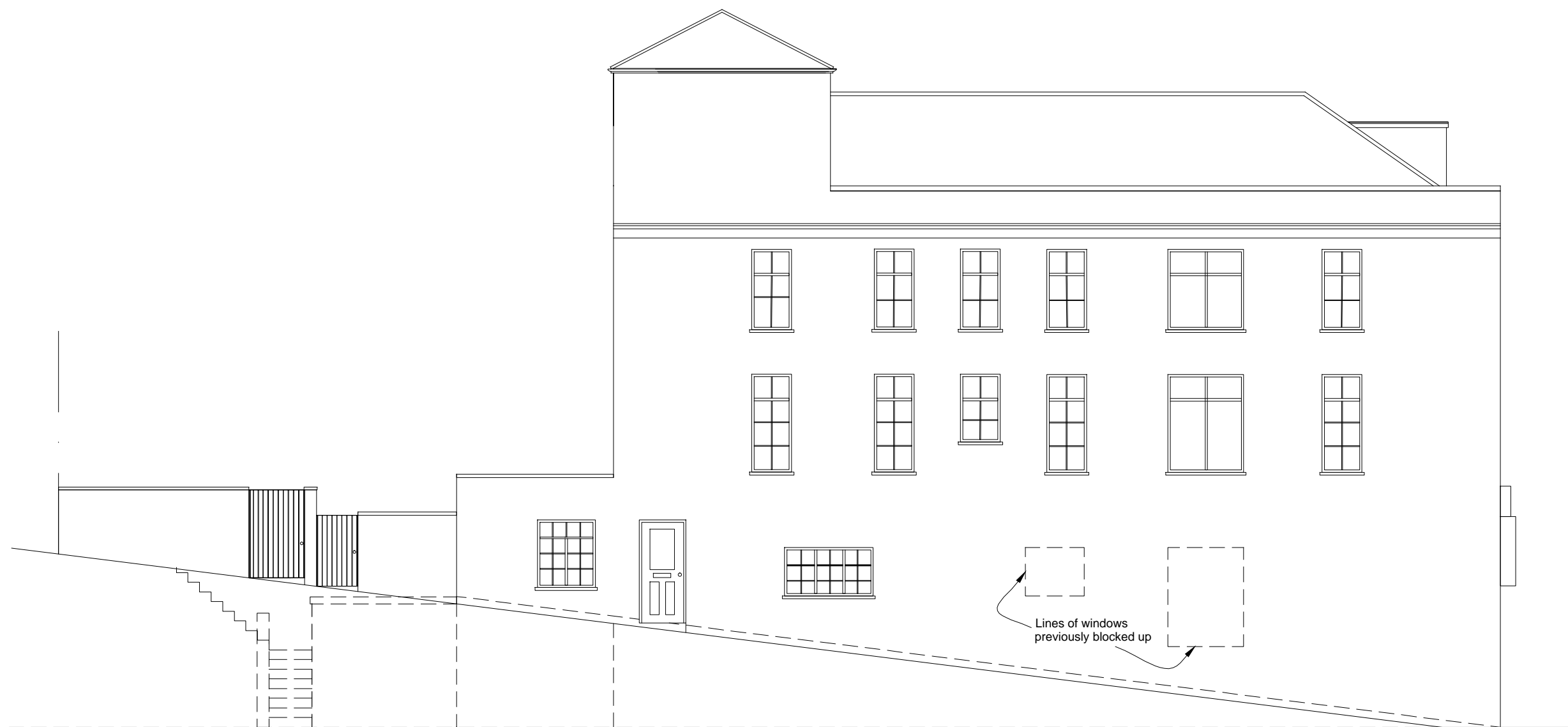
Proposed Side Elevation( Approved) 1:100
