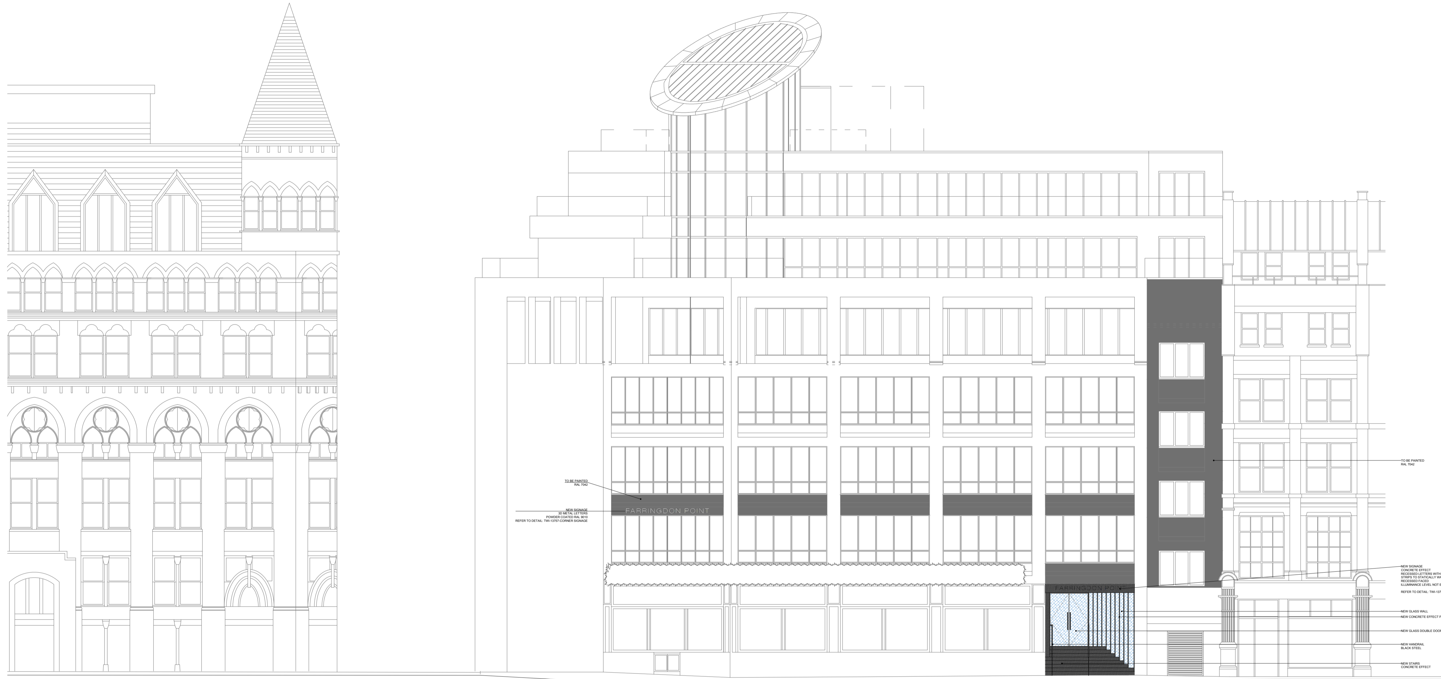
PROPOSED EAST ELEVATION SCALE: 1:100
