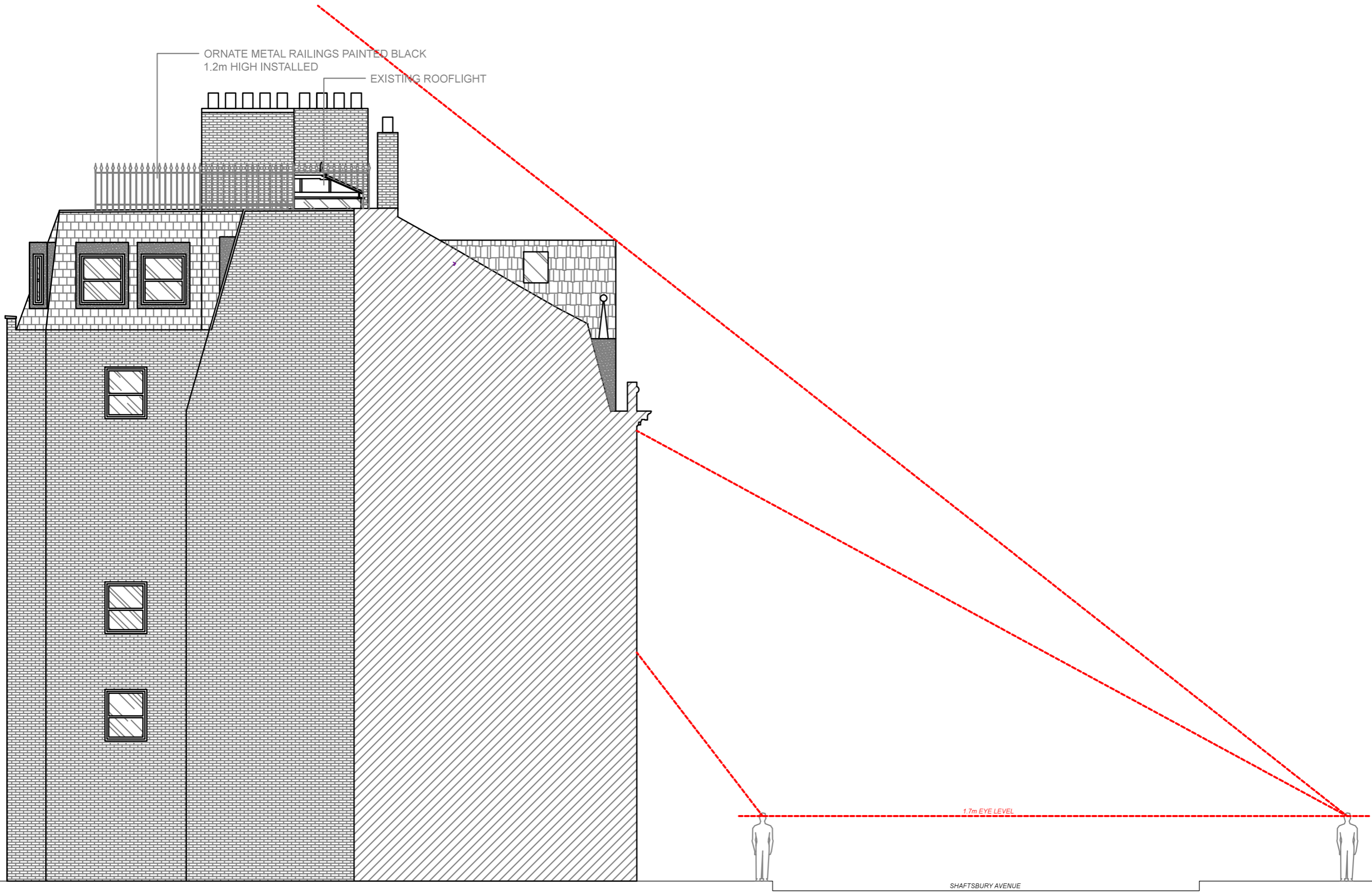
PROPOSED LEFT SIDE ELEVATION
