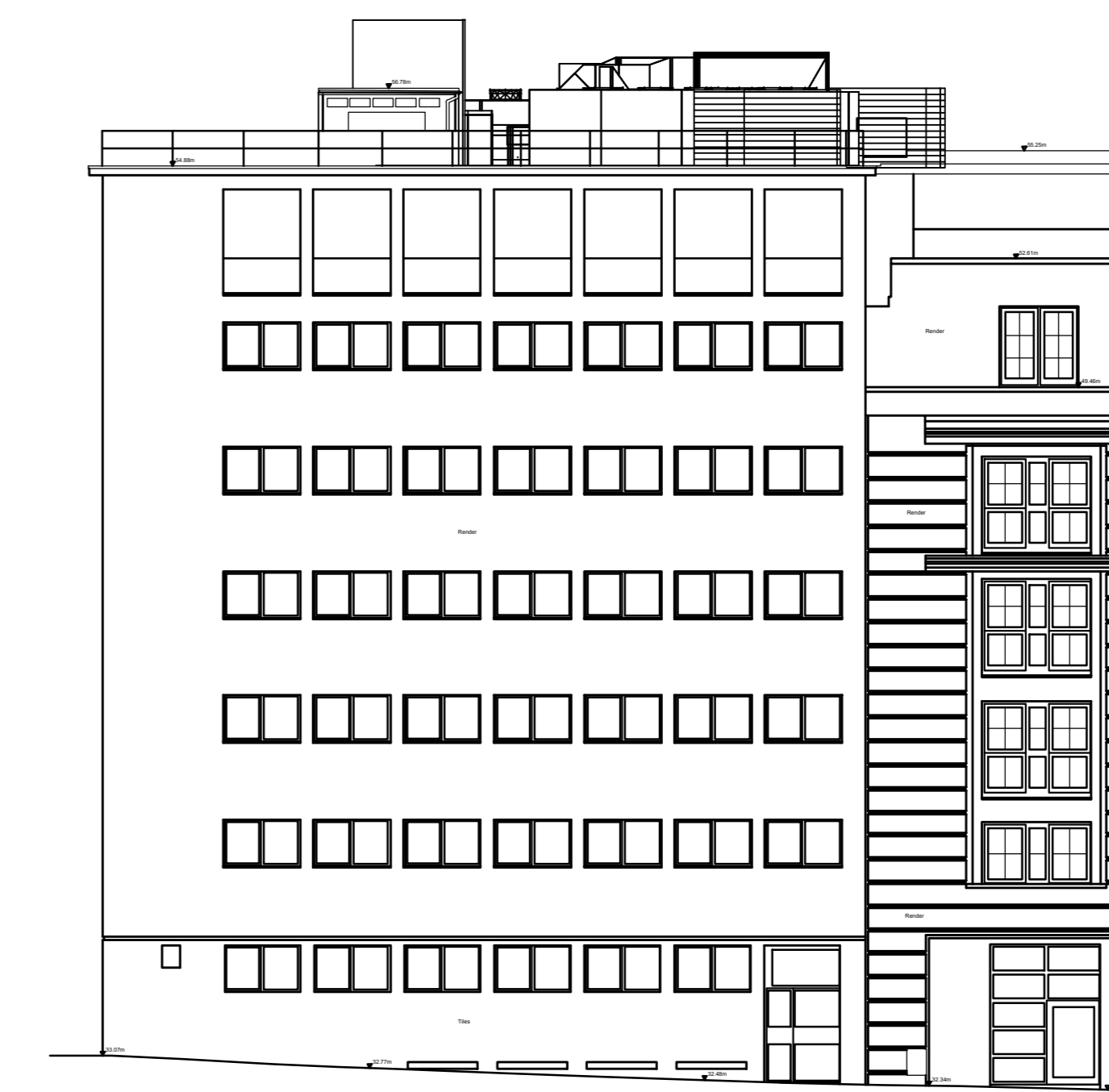
3 JAMESTOWN ROAD ELEVATION 1:150
