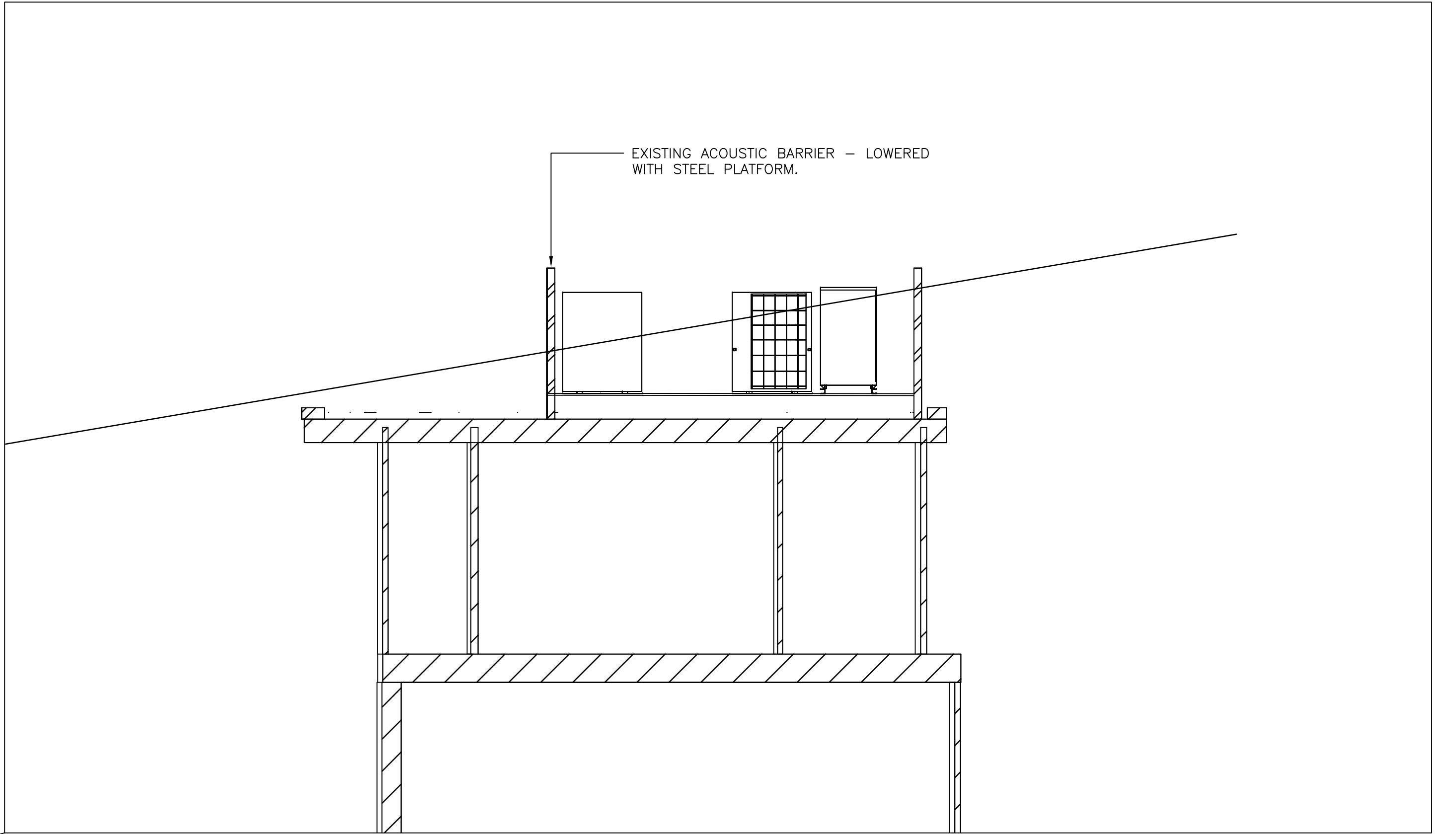
6: OVAL ROAD SIGHT LINE DETAIL SCALE 1:50
