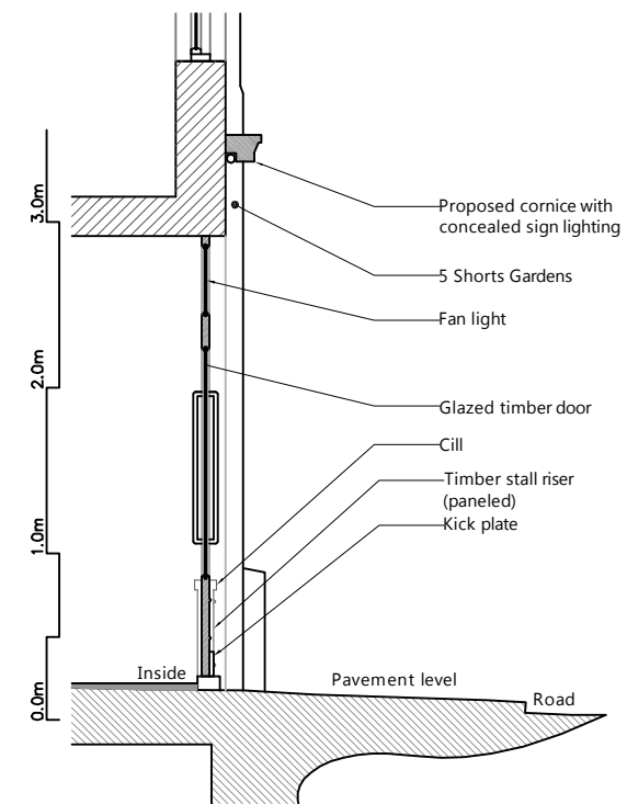
SECTION D-D AS PROPOSED @ 1:50 SCALE
