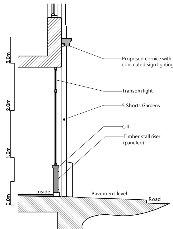
SECTION C-C AS PROPOSED @ 1:50 SCALE
