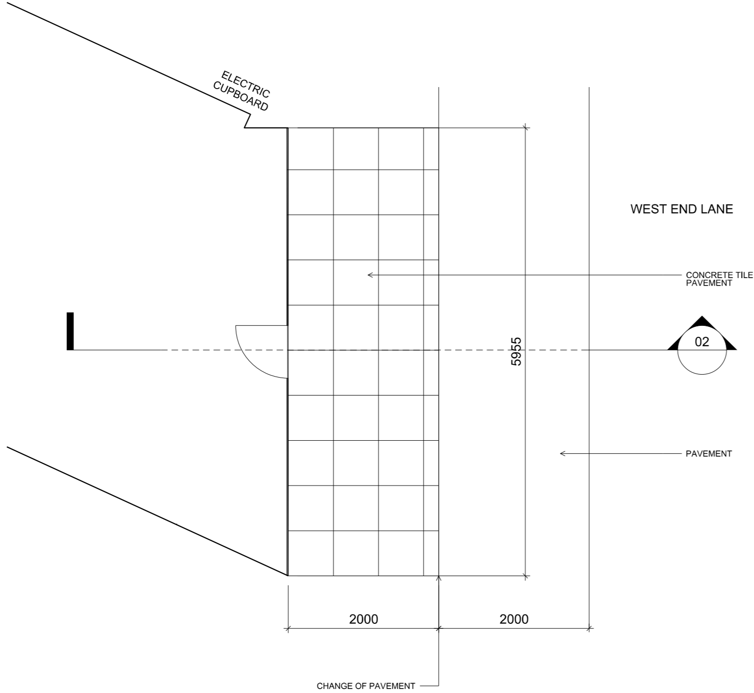
01 EXISTING FRONT GA LAYOUT 1:50
