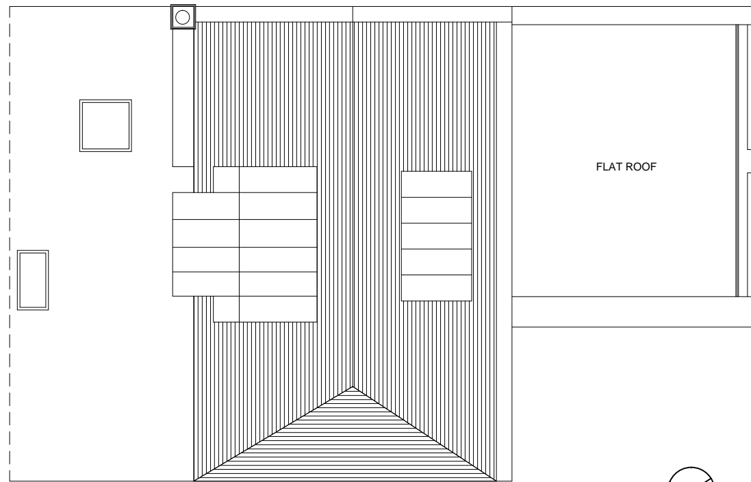
roof plan
