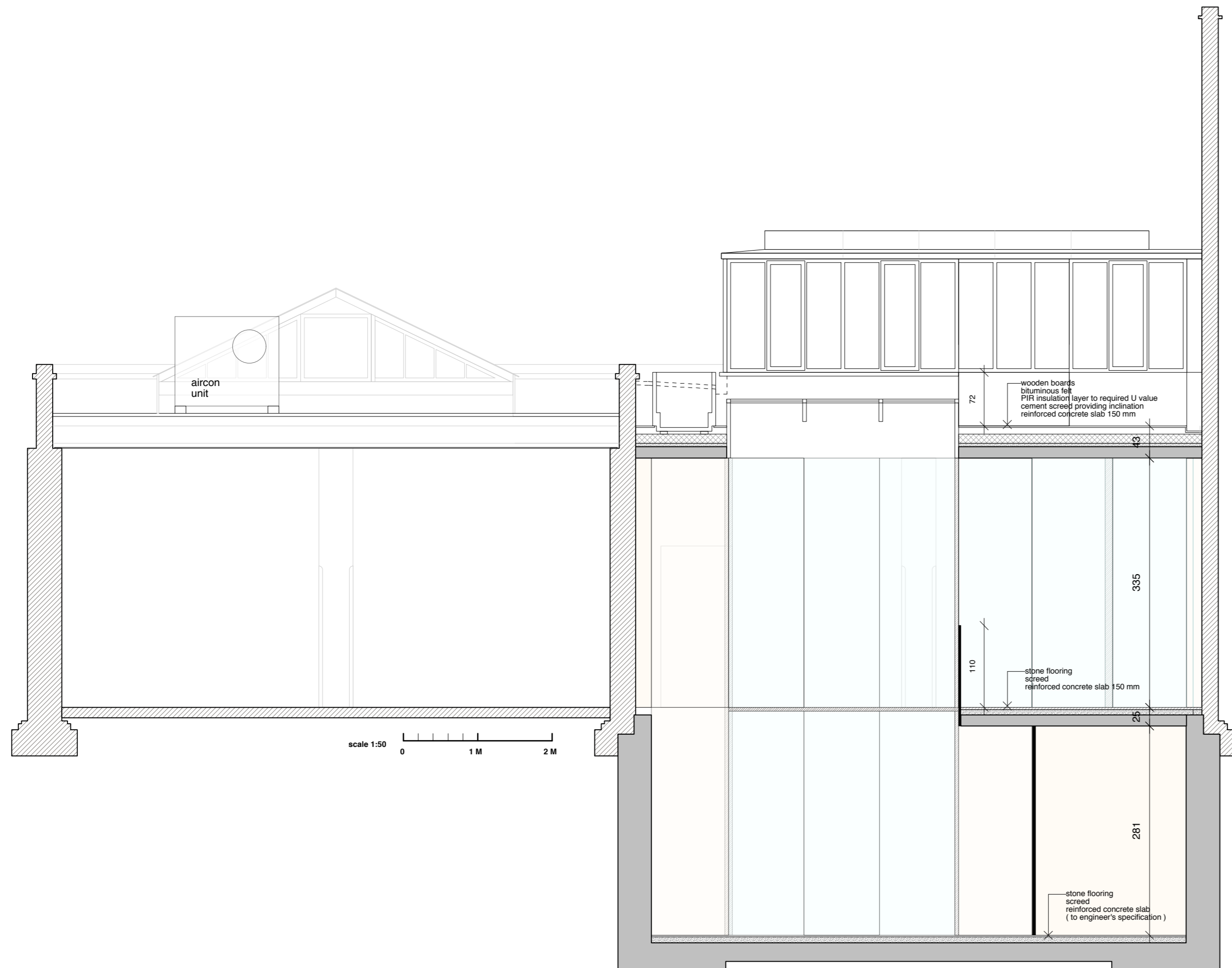
SECTION BB
