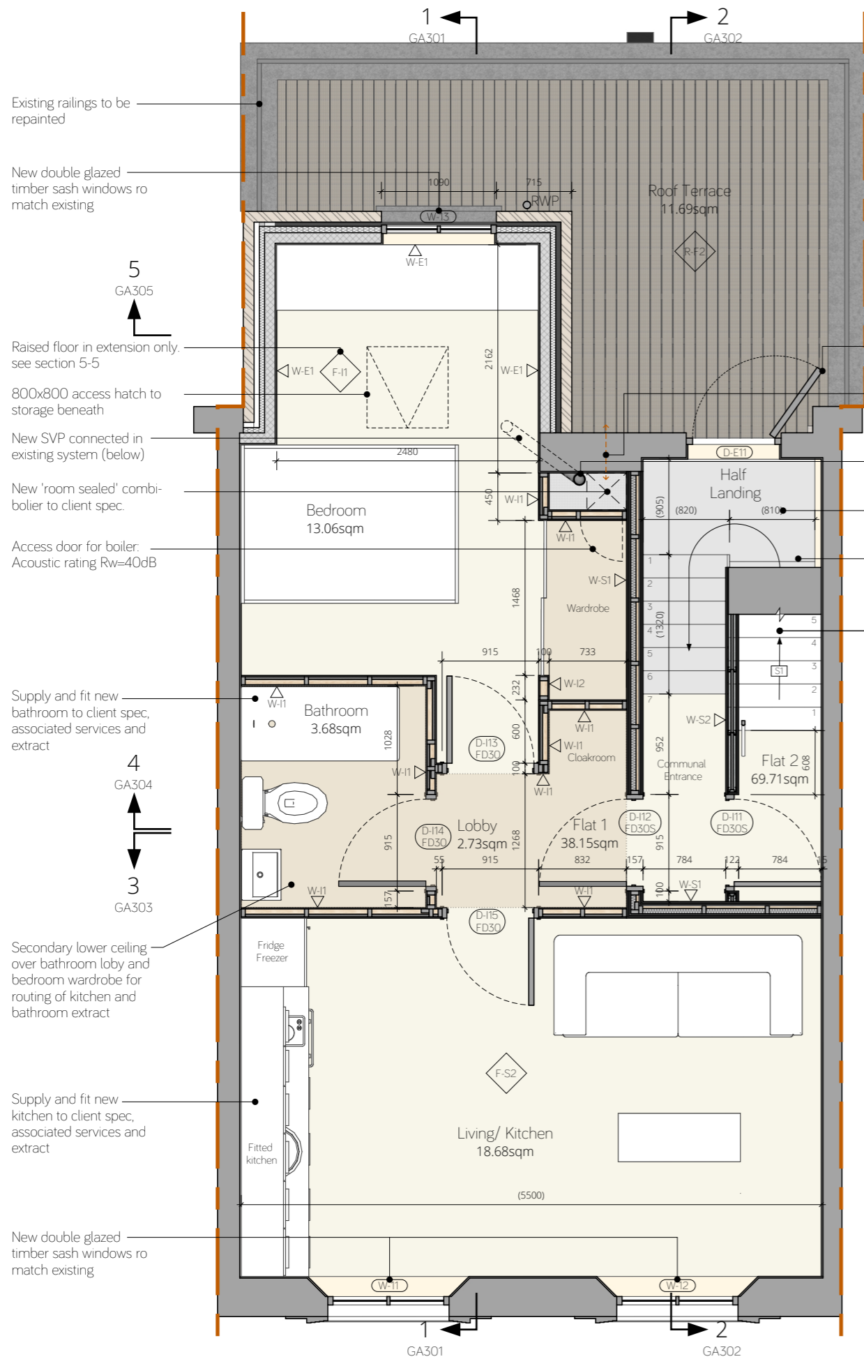
1st Floor (4.42sqm additional)
