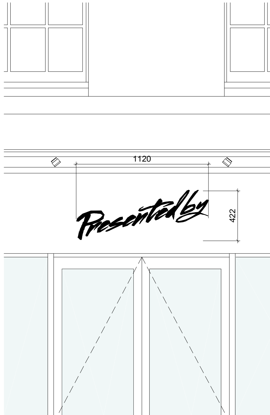
SHOPFRONT SIGNAGE @ 1:20
