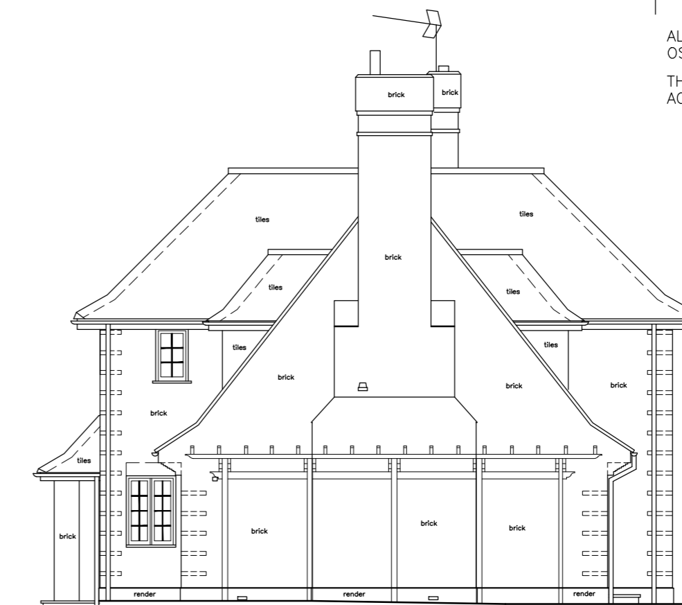
EAST ELEVATION
