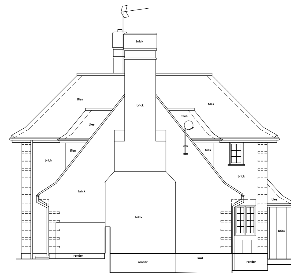
WEST ELEVATION
