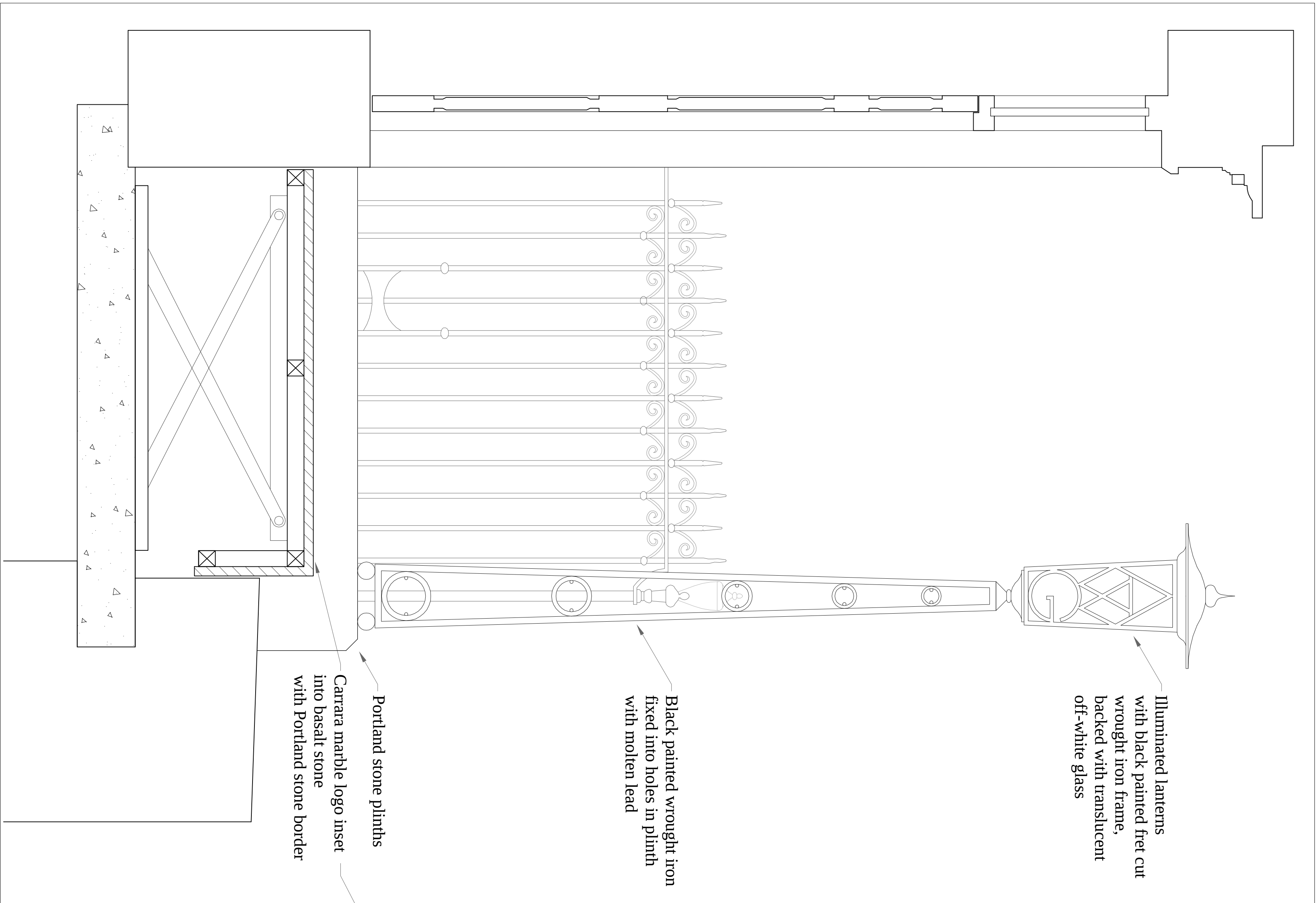
SECTION GG STEP IN STATIC POSITION scale 1:10 @ A1
