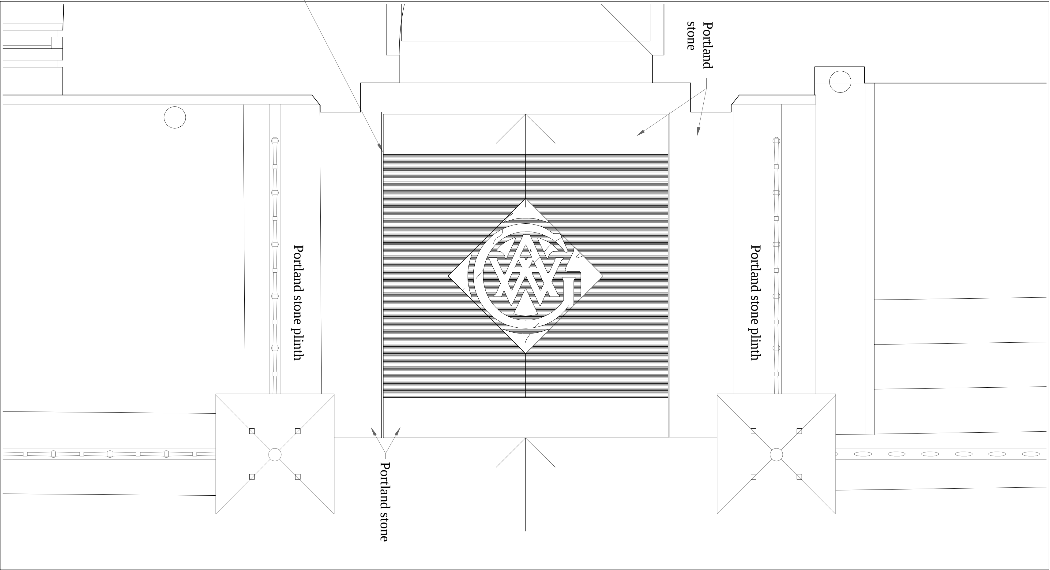
HYDRAULIC STEP PLAN scale 1:10 @ A1
