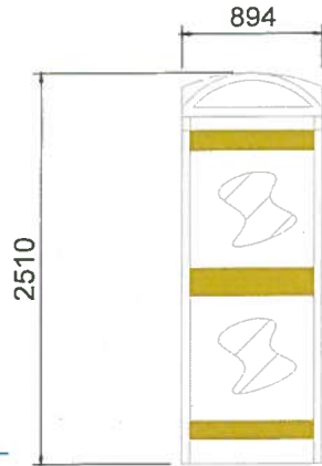
FRONT ELEVATION Scale 1:50
