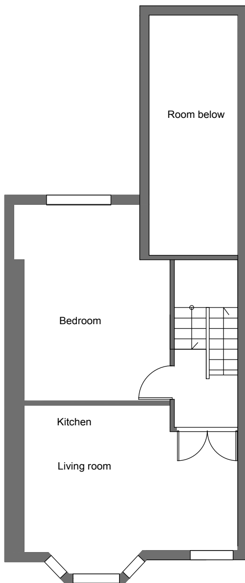
02 Proposed First Floor plan
