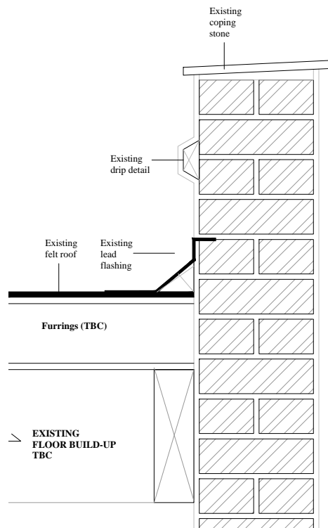
EXISTING PARAPET DETAIL @ 1:10
