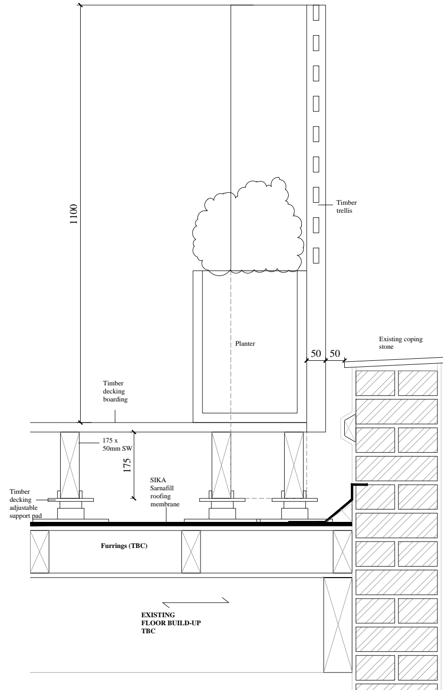
PROPOSED DETAIL A @ 1:10
