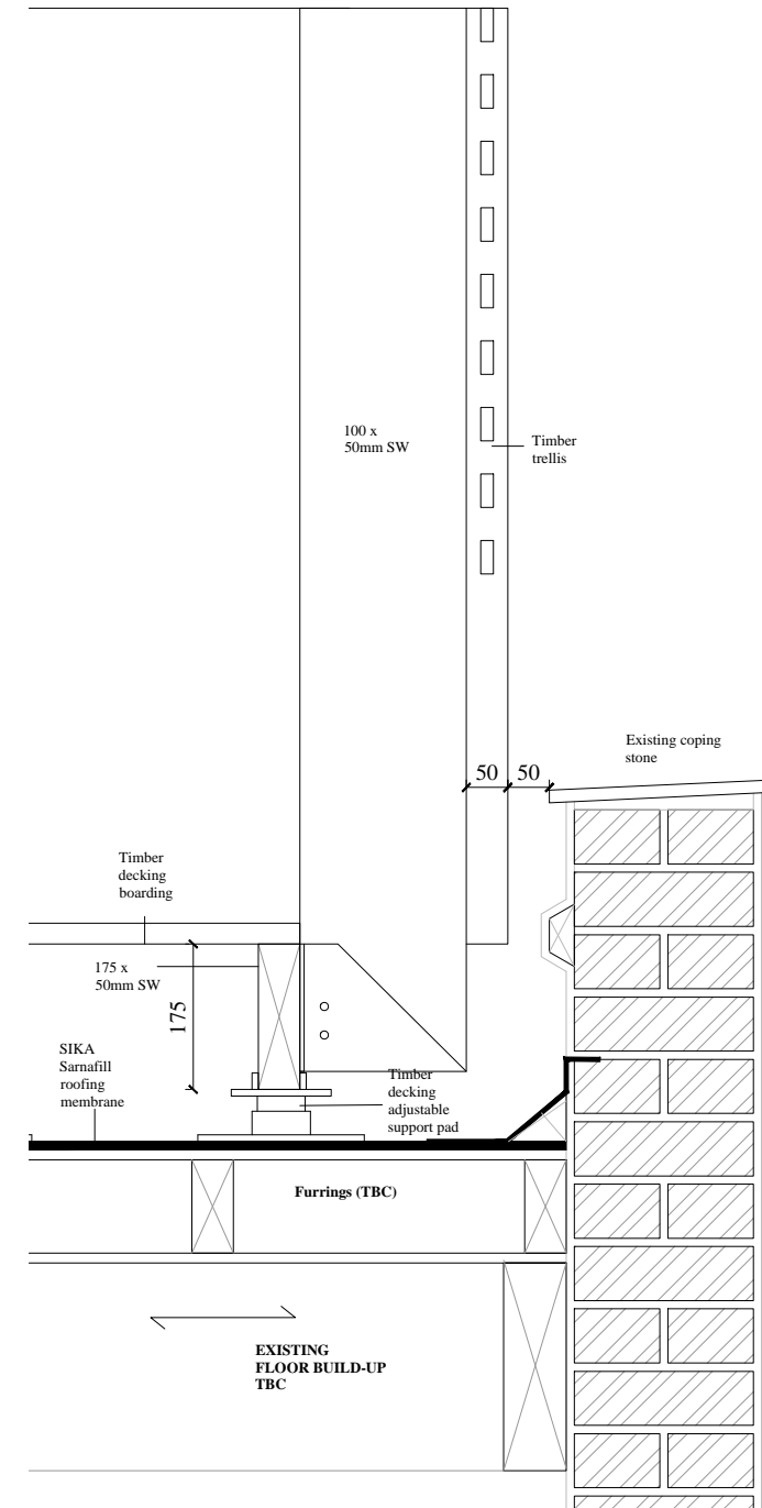
PROPOSED DETAIL B @ 1:10
