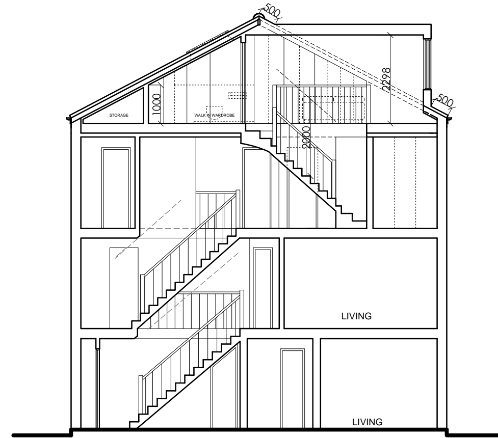
Section B-B
