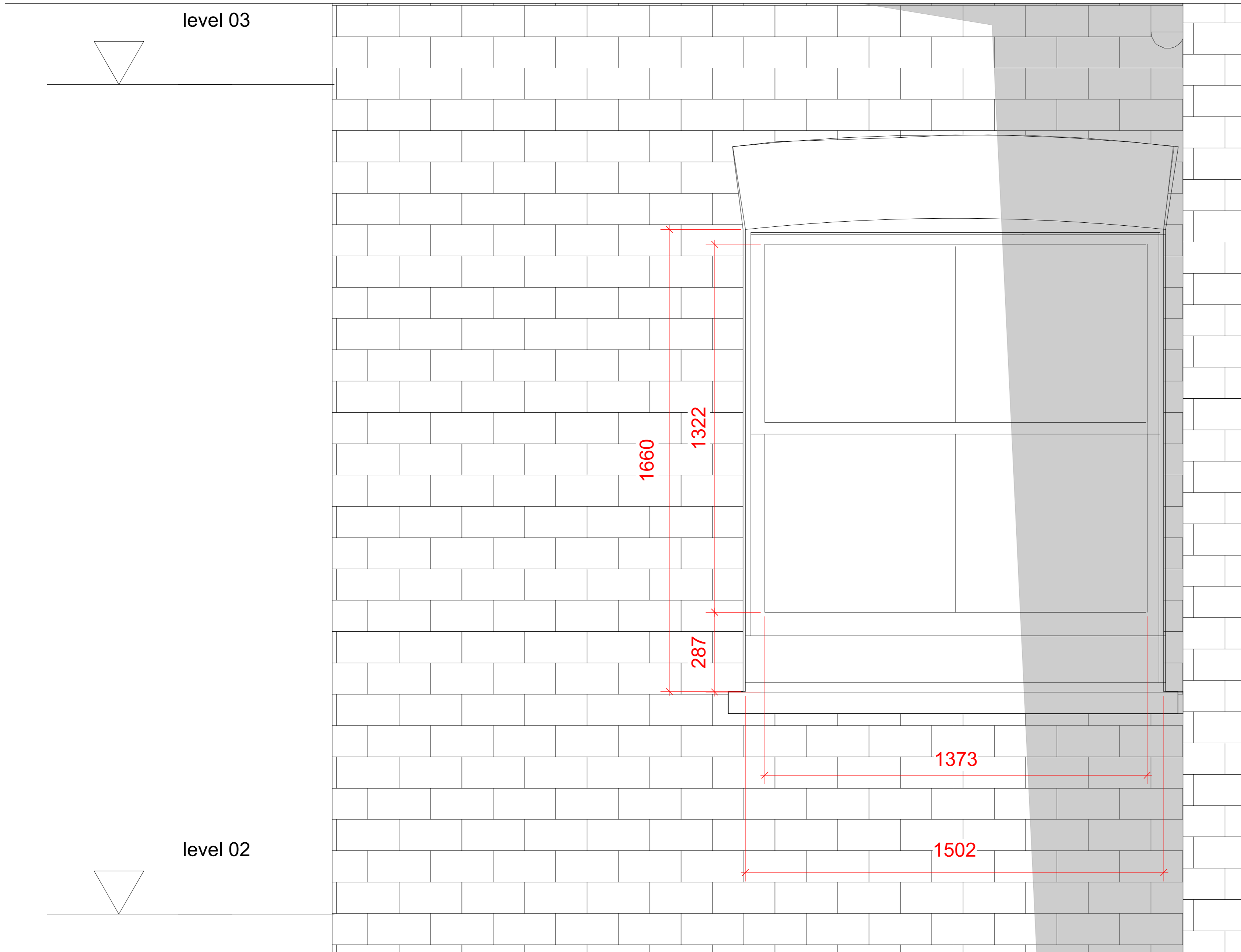
2 PROPOSED ELEVATION 02 Scale: 1:10
