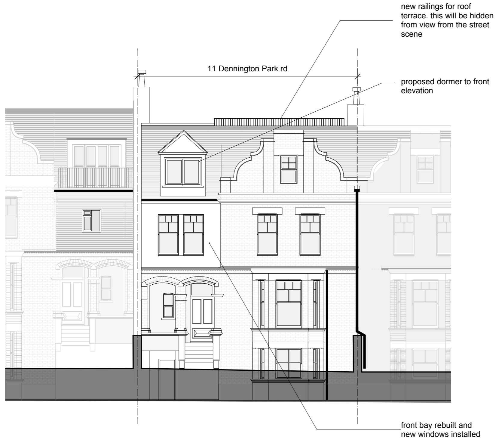
1 120 Proposed Front Elevation scale 1:100
