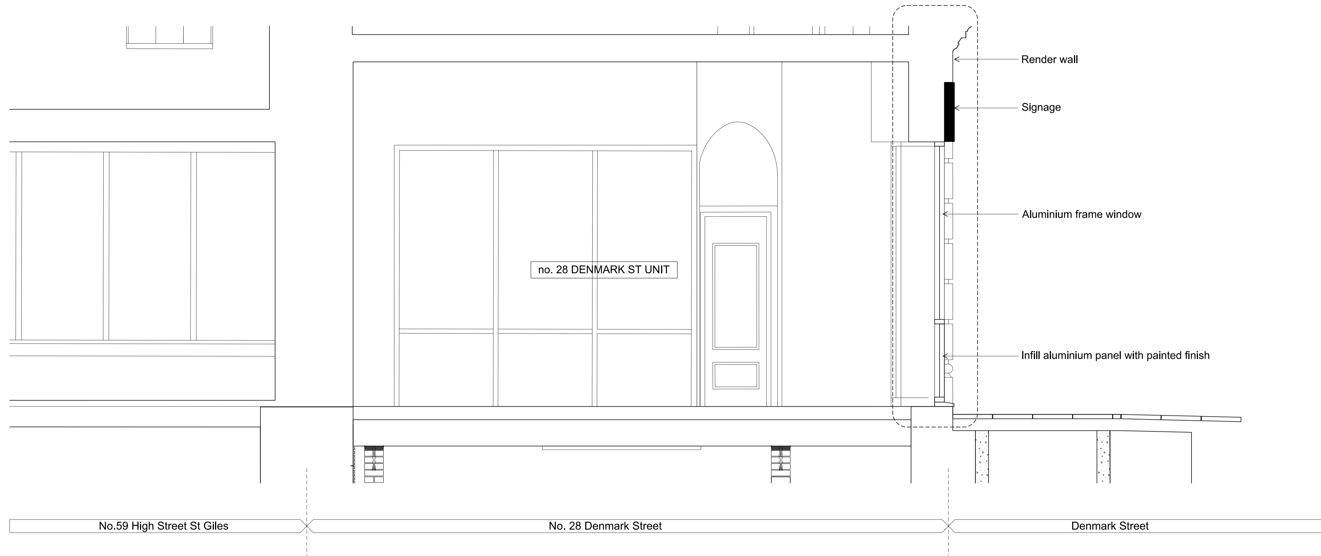
01 28 Denmark Street - Existing Ground Level Section 1:25
