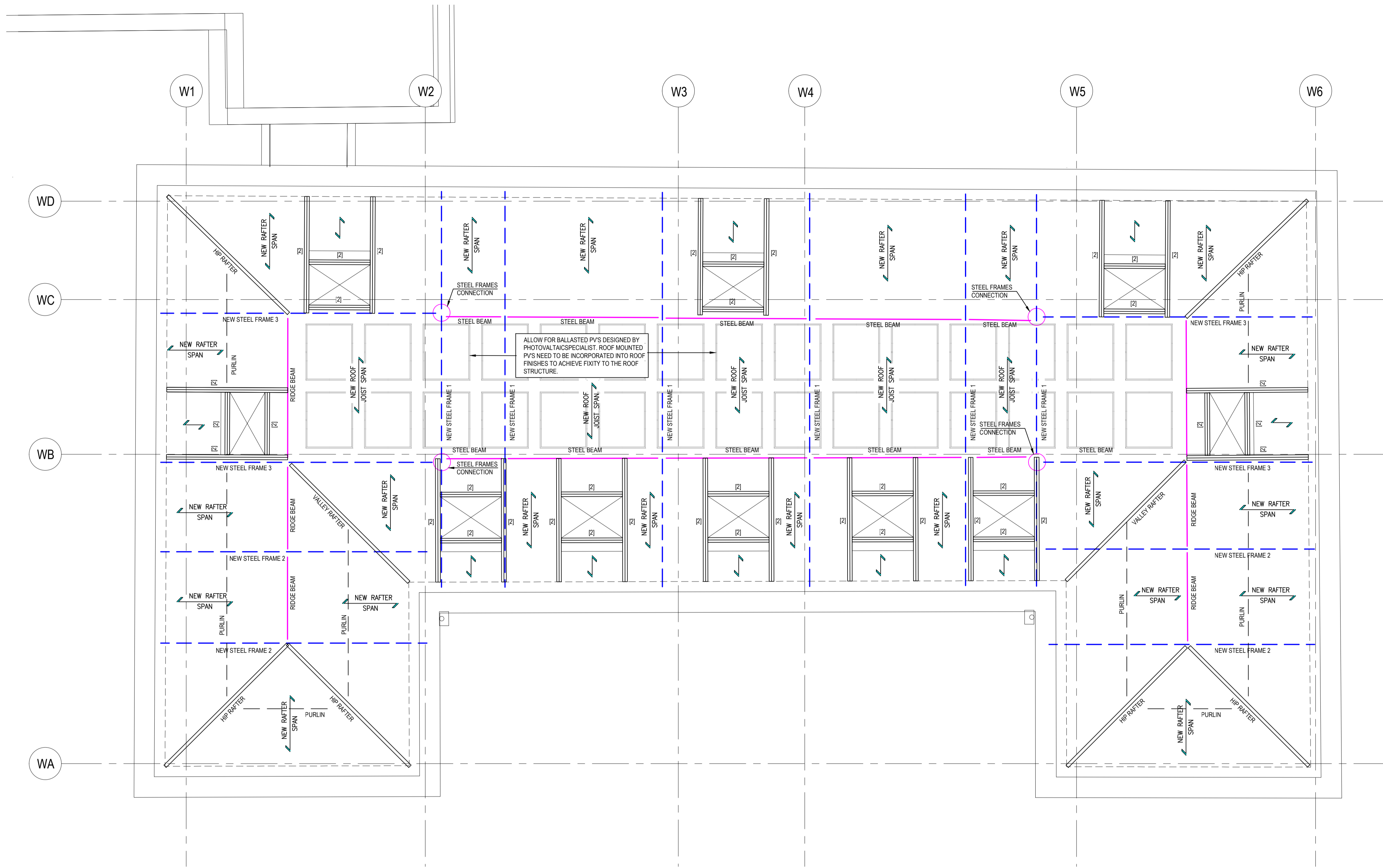
PROPOSED ROOF PLAN [ LEVEL RF ]
