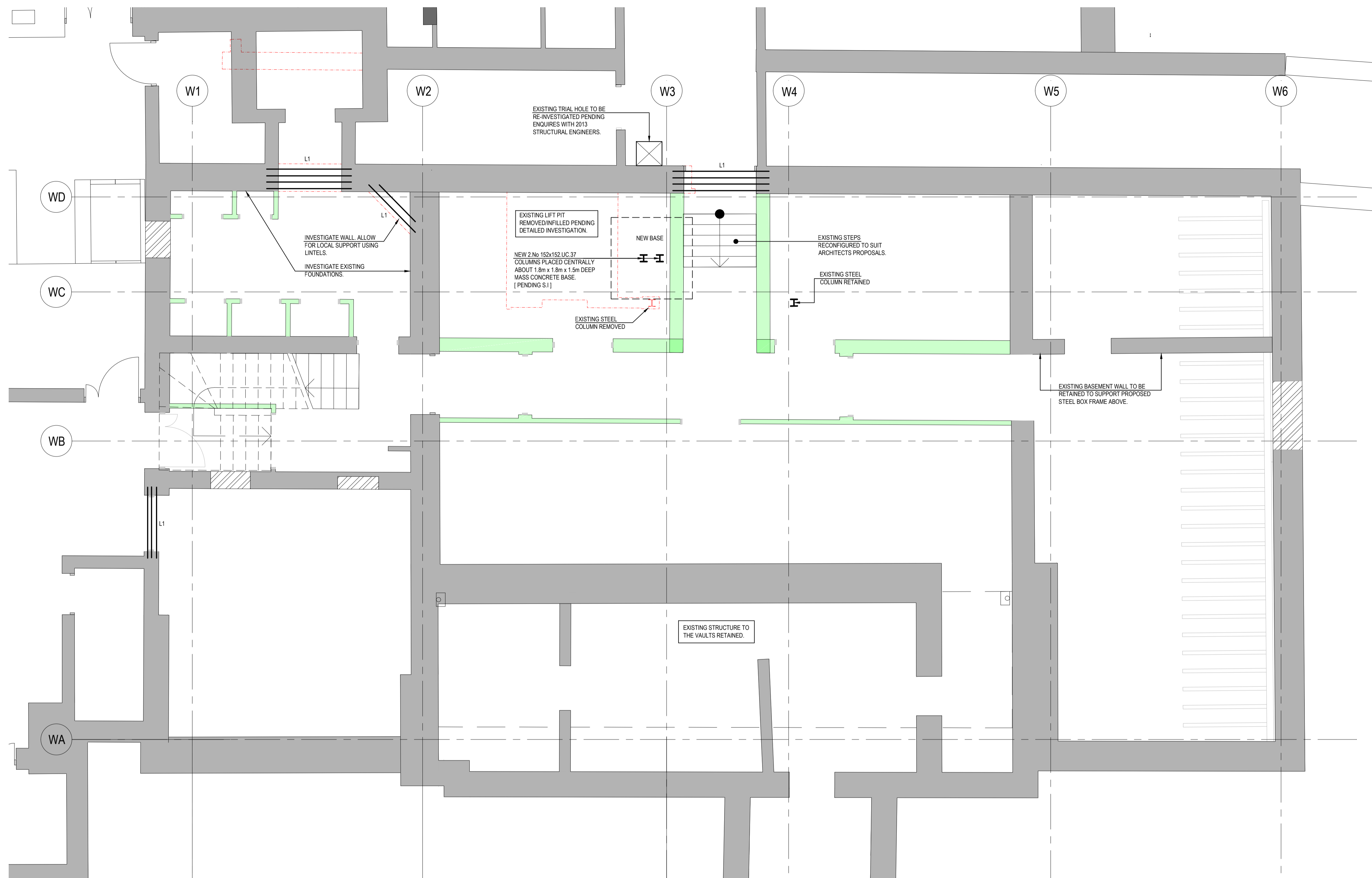
PROPOSED BASEMENT PLAN [LEVEL B1]
