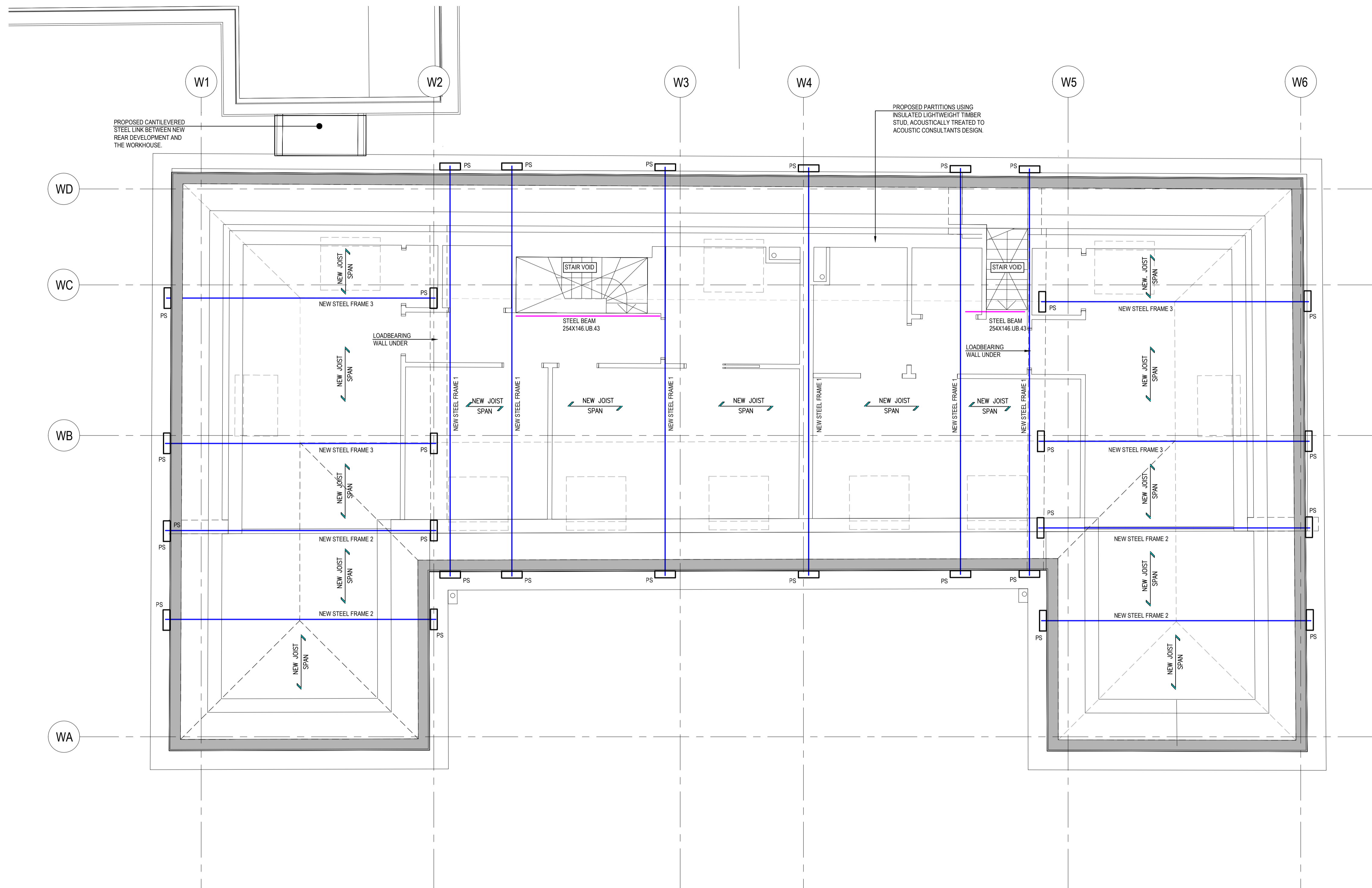
PROPOSED FOURTH FLOOR PLAN [ LEVEL 04 ]
