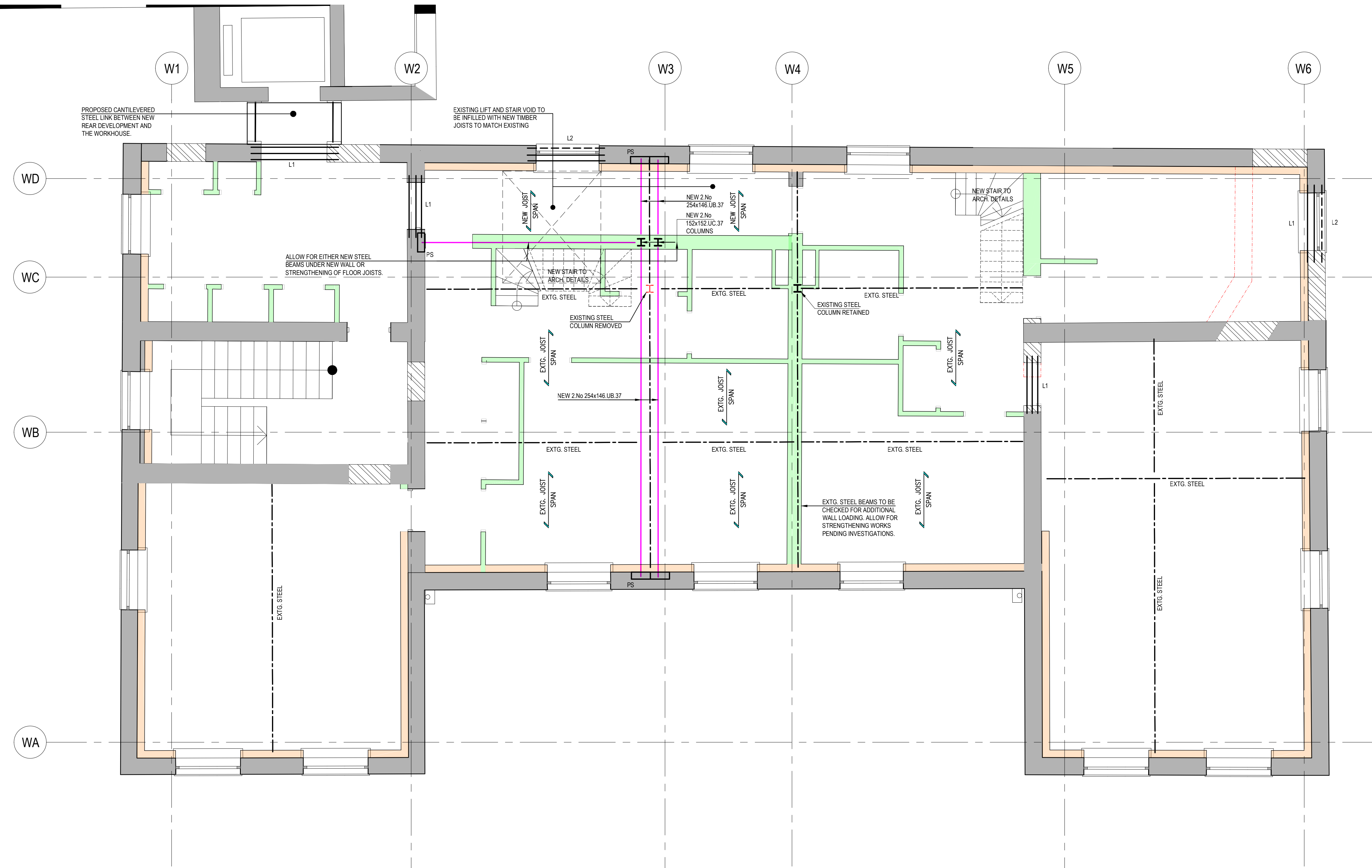
PROPOSED THIRD FLOOR PLAN [ LEVEL 03 ]
